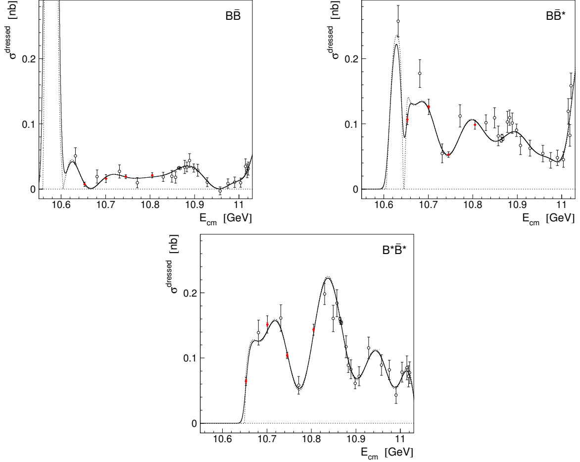
Figure 12. Energy dependence of the e^+e^- \rightarrow B\bar{B} (left), B\bar{B}^* (right), and B^*\bar{B}^* (bottom) cross sections. Red filled and black open circles show the Belle II and Belle measurements, respectively. In the Belle II results, black error bars show statistical uncertainties, red error bars show uncorrelated systematic uncertainties. (On six out of the twelve points, the systematic uncertainties are smaller than the size of the red filled circle, and thus not visible.) The solid curves show the default fit result; the dashed curves show the fit function before the convolution used to account for the E_{\text{cm}} spread.
