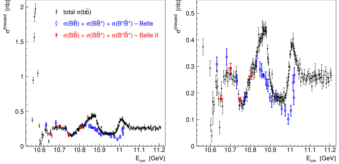
Figure 14. Energy dependence of the total b\bar{b} dressed cross section obtained in ref. [7] from the visible cross sections measured by Belle [31], and BaBar [26] (black circles) and the sum of the exclusive B\bar{B} , B\bar{B}^* , and B^*\bar{B}^* cross sections measured by Belle [8] (open blue circles) and in this work (filled red circles). The right panel shows the low cross-section region with an expanded scale.
