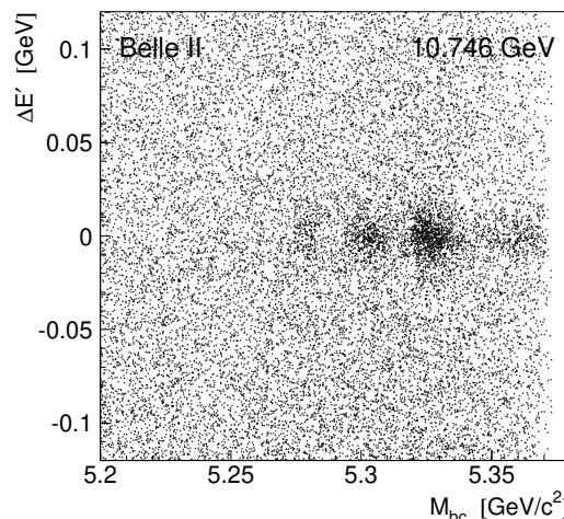
Figure 1. Distributions of \Delta E' vs. M_{bc} in the E_{cm} = 10.746 GeV data sample.
