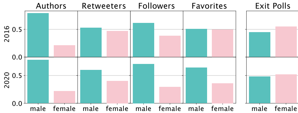
Figure 9. Gender distribution among social poll authors, their followers, as well as the retweeters and favoriters of the polls
