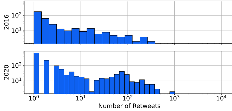
Figure 5. Histograms of the number of retweets per poll.
