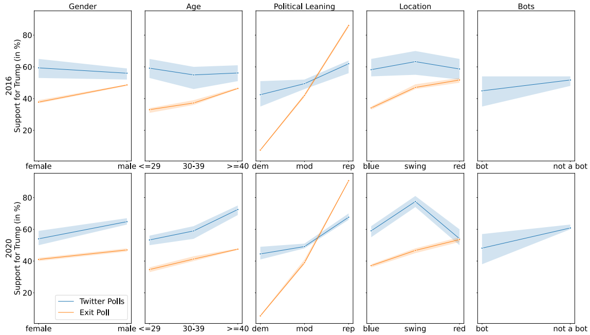
Figure 13. The average fraction of votes for Trump among Twitter polls authored by a user of certain inferred gender, age, and political affiliation (blue) in comparison to the fraction of votes for Trump in respective exit polls (orange).
