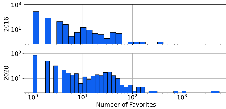
Figure 6. Histograms of the number of favorites per poll.
