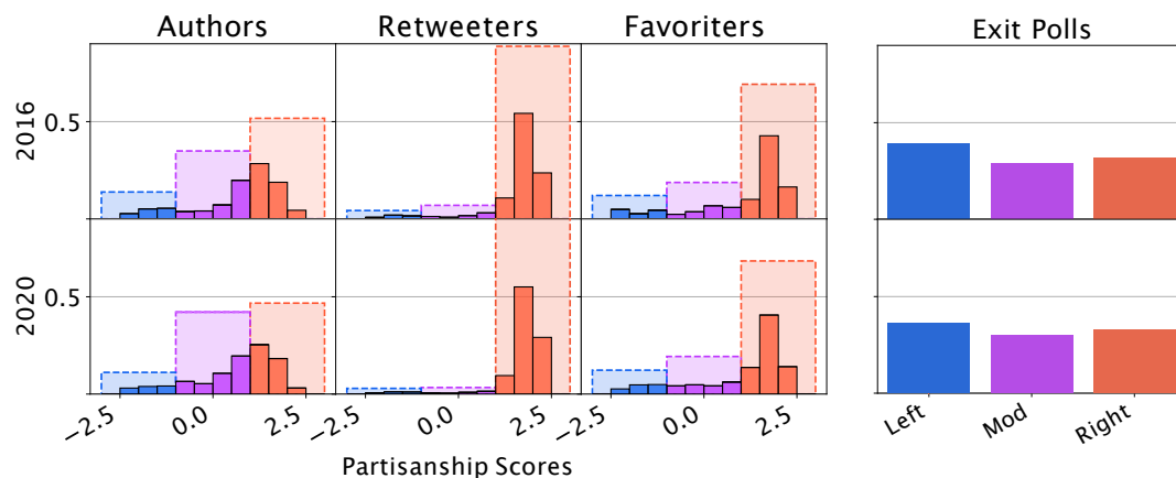
Figure 8. Political affiliation distribution of poll authors, retweeters, and favoriters
