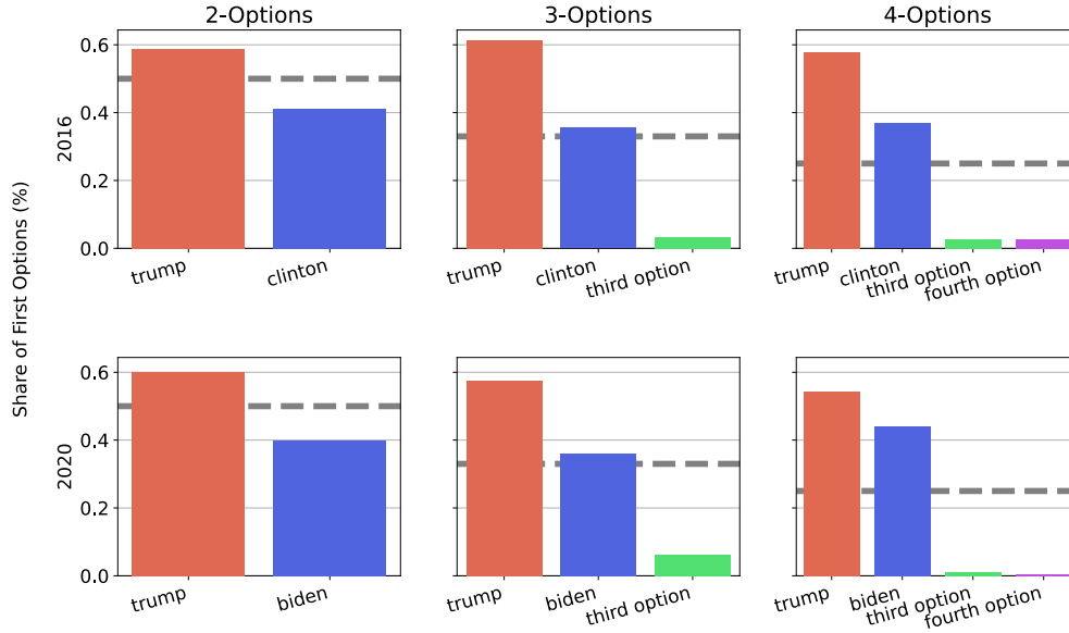
Figure 7. The fraction of Twitter polls listing a given candidate as first among the potential answers.
