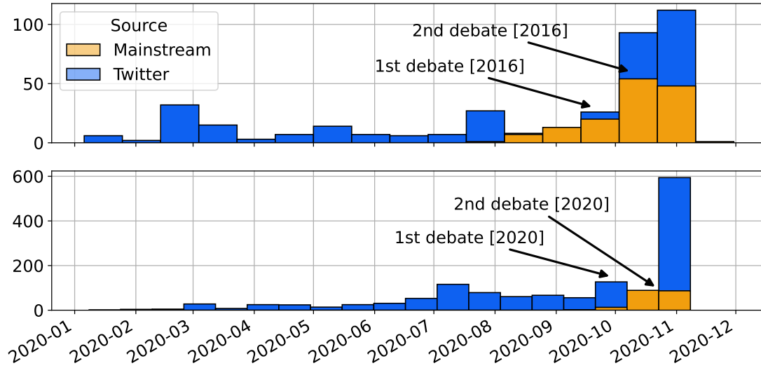
Figure 2. The number of Twitter and mainstream polls published over the course of the 2016 (top) and 2020 (bottom) U.S. presidential election years.
