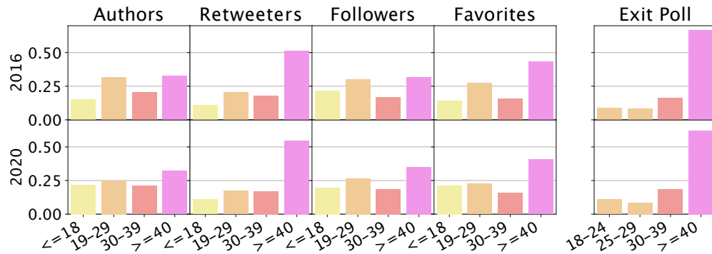
Figure 10. Age distribution of social poll authors, their followers, as well as the retweeters and favoriters of the polls.
