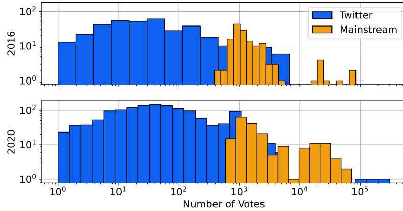
Figure 3. Distributions of the number of votes in Twitter and mainstream polls gauging support for the 2016 (top) and 2020 (bottom) U.S. presidential candidates.
