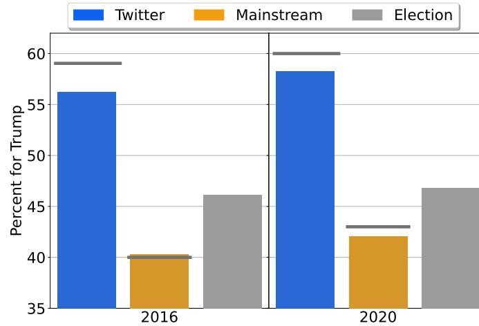
Figure 12. Average outcome of Twitter polls published before the 2016 and 2020 U.S. presidential election days the average outcomes of mainstream polls, and the official election outcomes.
