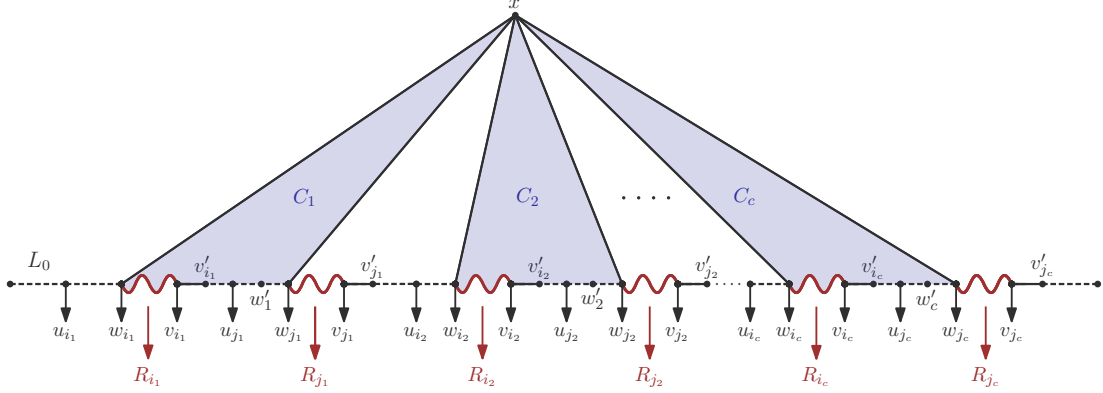
FIGURE 7. Proof of Lemma 4.3 (dashed lines depict paths of arbitrary length, and highlighted paths have length at least h ).
