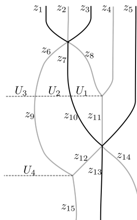
Figure 16. The space \mathbb{V}^{\mathfrak{w}} for this algebraic weave \mathfrak{w} is \mathbb{C}^{15} \times (\mathbb{C}^{\binom{3}{2}} \times (\mathbb{C}^*)^3)^4 . Indeed, there are 15 weave segments, each labeled with a variable z_i \in \mathbb{C} , and 4 dashed segments, each labeled with an invertible triangular matrix U_j . The correspondence \mathcal{M}(\mathfrak{w}) associated to this algebraic weave is a closed subvariety of \mathbb{V}^{\mathfrak{w}} .
