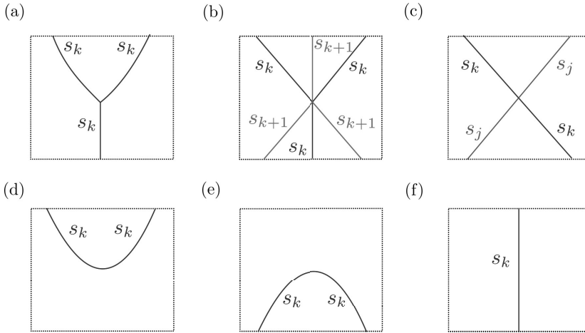
Figure 8. The six local models for sliced n -weave. In (a), (c), (d), (e), and (f), we have j, k \in [1, n-1] . In (b), we have k \in [1, n-2] , and |j-k| \geq 2 . The inverse of the local model in (b), with s_{k+1}s_k s_{k+1} on top and s_k s_{k+1} s_k on the bottom, is also allowed.
