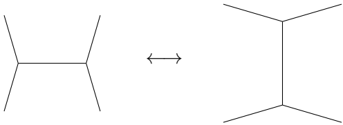
Figure 7. Weave mutation, after [25, Theorem 4.21]. This is not an equivalence.
