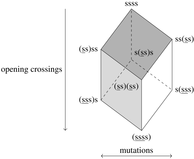
Figure 9. The Hasse graph of the Boolean lattice 2^{[3]} . The top vertex is the initial braid word \beta \cdot \Delta = s^3 \cdot s = s^4 , the bottom vertex represents \Delta = s . Demazure weaves \mathfrak{w} \in \text{Hom}_{\mathfrak{M}_2}(ssss, s) correspond to monotone paths from the top vertex to the bottom vertex.
