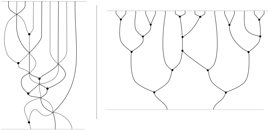
Figure 5. (Left) A 3-weave from \beta_2 = (\sigma_1 \sigma_2)^4 \sigma_1 \in Br_3^+ down to \beta_1 = \sigma_2 \sigma_1 \sigma_2 \in Br_3^+ . The darker shade indicates a transposition label s_1 \in S_3 and the lighter shade indicates the transposition label s_2 \in S_3 . (Right) A 2-weave from \beta_2 = \sigma_1^{16} \in Br_2^+ to \beta_1 = \sigma_1^2 \in Br_2^+ , all black edges are labeled with the unique transposition s_1 \in S_2 . Trivalent vertices are emphasized in orange in both weaves.
