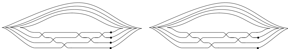
Figure 3. The front ( xz ) projection of the rainbow closure of the braid word \beta = \sigma_1 \sigma_2 \sigma_3 \sigma_1 \sigma_2 \sigma_1 , with one marked point per strand (left) and one marked point per component (right). This is a braid word for the half-twist \Delta_4 . Note that the Legendrian condition implies that all crossings are overcrossings. Note also that the marked points are located to the right of all crossings of \beta .
