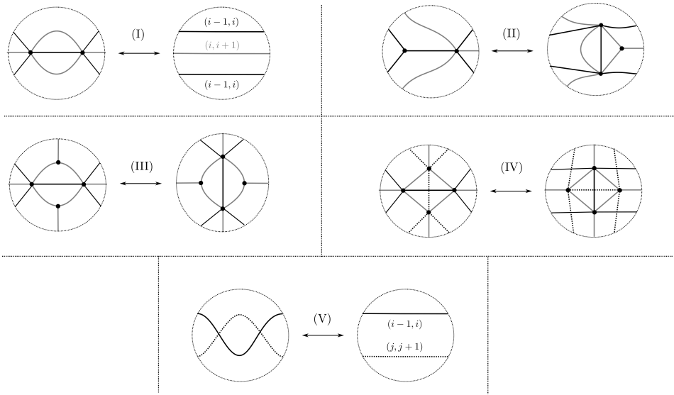
Figure 6. Weave equivalences, after [25, Theorem 1.1].
