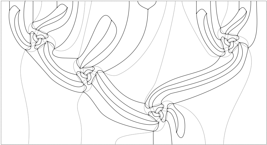
Figure 1. An algebraic weave in \mathrm{Hom}_{\mathfrak{W}_n}(\gamma, \gamma') between the two positive 3-braids \gamma = \sigma_1^3\sigma_2\sigma_1^3\sigma_1^2\sigma_1^3\sigma_2^3\sigma_1^3\sigma_2\sigma_1^3 , at the top, and \gamma' = \sigma_2^3\sigma_1^2\sigma_2^3 , at the bottom. The darker shade is labeled with the transposition s_1 and the lighter shade is labeled with s_2 . For readability we omit the (downward pointing) orientations. The upside-down trivalent vertices are defined using the usual trivalent vertices and cups, see Section 4.3.2.
