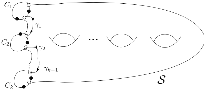
Figure 4. The surface \mathcal{S} , with the marked points in the boundary. Points of A are colored white, and points of B are colored black. For the sake of readability we do not label the paths along the boundary for two consecutive points of A .
