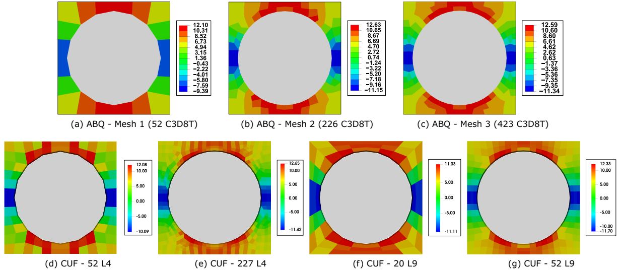
Figure 5: Distribution of residual stress (22-component) in the square-packed RUC at the end of cure.
