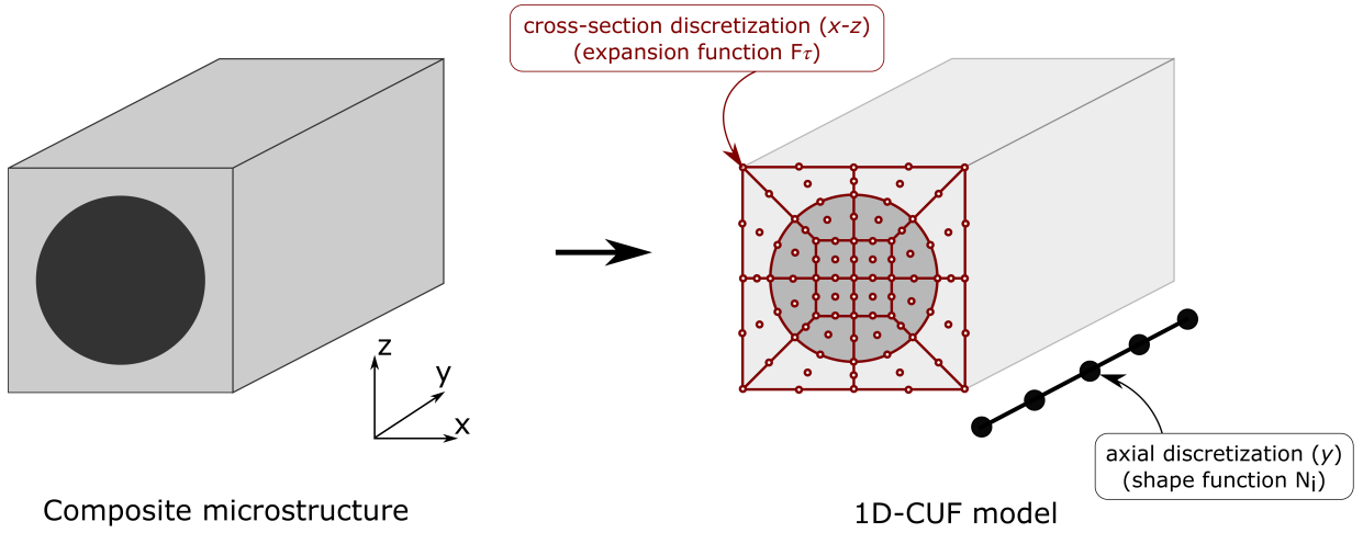
Figure 2: Modeling of a prismatic structure using 1D-CUF.
