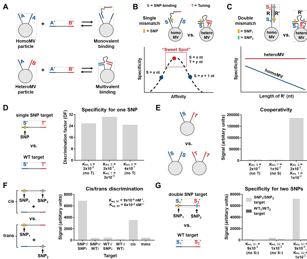
Figure 1. Hypothesized advantages of heteromultivalent DNA hybridization and modeling key applications.
