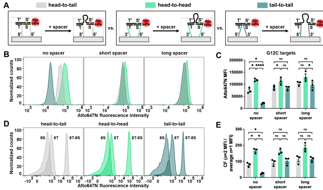
Figure 4. Determining the impact of binding orientation on heteromultivalent binding specificity and cooperativity. (a) Scheme describing n=2 beads with head-to-tail, head-to-head, or tail-to-tail orientation binding to targets with or without a spacer region. (b) Representative histograms for 8T-8S beads with each orientation binding the G12C no spacer, short spacer, and long spacer targets. (c) Measured median fluorescence intensity values for 8T-8S beads with each orientation binding the G12C target with no spacer, short spacer, and long spacer targets. (d) Representative histograms for 8T, 8S, and 8T-8S beads with each orientation binding the G12C no spacer target. (e) Measured cooperativity factors for 8T-8S beads with each orientation binding the G12C no spacer, short spacer, and long spacer targets. Error bars represent standard error of the mean. Values were compared using paired one-way ANOVA with multiple comparisons follow-up tests ( ^{ns}P > 0.05 , ^{*}P < 0.05 , ^{****}P < 0.0001 ).
