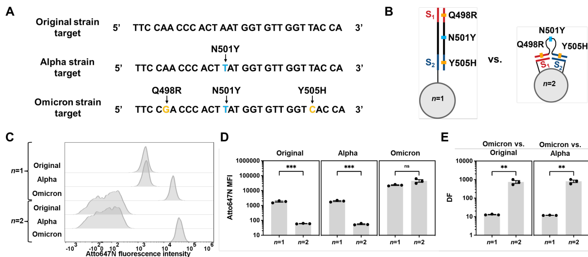
Figure 6. Distinguishing different strains of SARS-CoV-2 using heteroMV hybridization. (a) Sequences of targets based on the original, alpha, and omicron strains of SARS-CoV-2 spike protein, with the mutations in each target indicated with arrows. (b) Scheme describing the binding of an n=1 bead functionalized with an oligo that is fully complementary to the omicron target and the binding of an n=2 bead functionalized with S_1 and S_2 oligos that are complementary to the regions of the target containing the Q498R and Y505H mutations but not the N501Y mutation. (c-d) Representative histograms (c) and measured median fluorescence intensity values (d) for the n=1 and 8 S_1 -9 S_2 n=2 beads binding each target. (e) Measured discrimination factors for the n=1 and 8 S_1 -9 S_2 n=2 beads binding the omicron target vs. the original target or the omicron target vs. the alpha target. Values were compared using unpaired student t tests ( ^{ns}P > 0.05 , ^{**}P < 0.01 , ^{***}P < 0.001 ). Error bars represent standard error of the mean.
