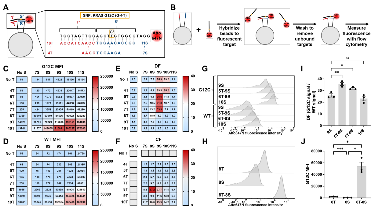
Figure 2. Measuring the specificity and cooperativity of heteromultivalent binding using flow cytometry. (a) Design of the oligonucleotides included in the screen to maximize discrimination factor and best cooperativity factor. Yellow box indicates the position of the SNP in the target sequence. (b) Scheme describing the flow cytometry-based assay used to quantify target binding to 5 \mu m DNA-coated silica particles. (c and d) Heatmaps showing the median fluorescence intensity of each bead included in the screen when incubated with the G12C target (c) and the WT target (d). (e and f) Heatmaps showing the discrimination factor (e) and cooperativity factor (f) of each bead included in the screen. The cooperativity factor is shown for beads incubated with the G12C target. (g) Representative histograms for 9S, 5T-9S, 6T-9S, and 10S beads binding the G12C and WT targets. (h) Representative histograms for 8T, 8S, and 8T-8S beads binding the G12C target. (i) Measured discrimination factors for 9S, 5T-9S, 6T-9S, and 10S beads. (j) Measured median fluorescence intensity values for 8T, 8S, and 8T-8S beads binding the G12C target. Error bars represent standard error of the mean. Values were compared using paired one-way ANOVA with multiple comparisons follow-up tests ( ^{ns}P > 0.05 , ^*P < 0.05 , ^{**}P < 0.01 , ^{***}P < 0.001 ).
