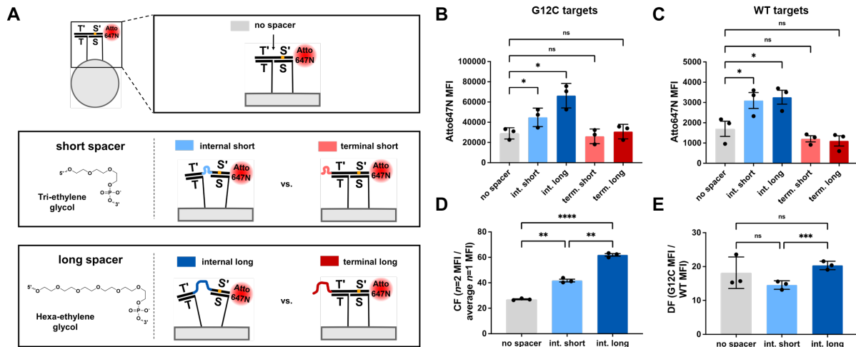
Figure 3. Determining the impact of spacer length on heteromultivalent binding. (a) Scheme describing the design of the no spacer target, the internal and terminal short spacer targets, and the internal and terminal long spacer targets including the chemical structures of the PEG spacer molecules. (b and c) Measured median fluorescence intensity values for 8T-8S beads binding the G12C (b) and the WT (c) no spacer, internal short spacer, internal long spacer, terminal short spacer, and terminal long spacer targets. (d and e) Measured cooperativity factors (d) and discrimination factors (e) for the 8T-8S beads binding the G12C target containing no spacer, the internal short spacer, or the internal long spacer. Error bars represent standard error of the mean. Values were compared using paired one-way ANOVA with multiple comparisons follow-up tests ( ns P > 0.05, *P < 0.05, **P < 0.01, ***P < 0.001, ****P < 0.0001).
