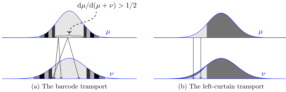
FIG. 1. Comparison of the barcode transport and the left-curtain transport for Gaussian marginals. (a) The barcode transport consists of a collection of left-curtain transports represented by different shades. The map h follows the reverse of the indicated arrows. (b) The left-curtain transport is the identity on the light-gray area and does not admit a (backward) Monge map there.
