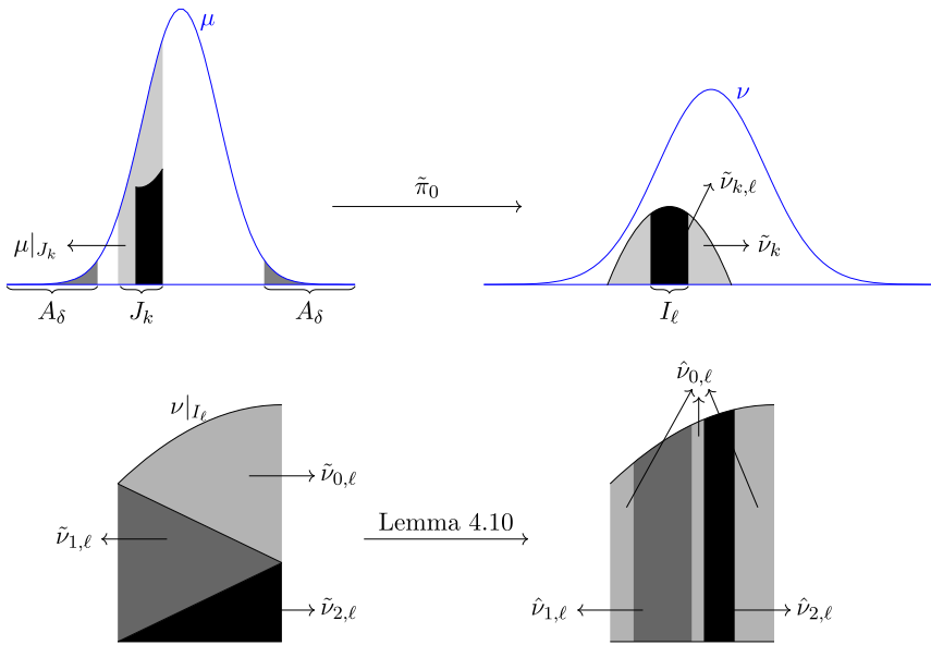
FIG. 7. Illustrating the transport \tilde{\pi}_0 and Lemma 4.10.
