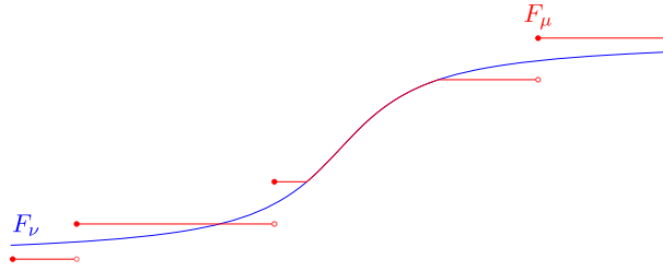
FIG. 2. Distribution functions of \mu, \nu where the MMT (and MT) from \mu to \nu is unique.
