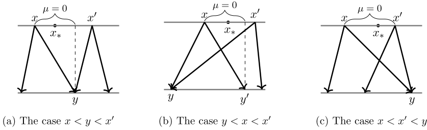
FIG. 4. Illustration of the three cases.
