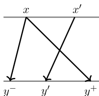
FIG. 3. Forbidden configuration for left-monotonicity: the legs of a point x' cannot step into the legs of another point x to the left of x' .
