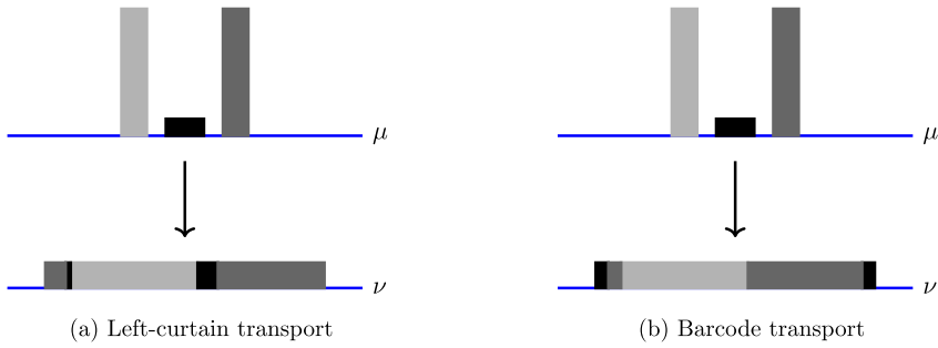
FIG. 6. Left-curtain and barcode transport are MMTs, yet do not coincide.
