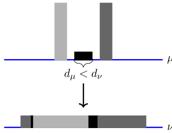
FIG. 5. The left-curtain transport \pi_{1c} is not the identity on \{x \in \mathbb{R} : d_\mu(x) < d_\nu(x)\} .
