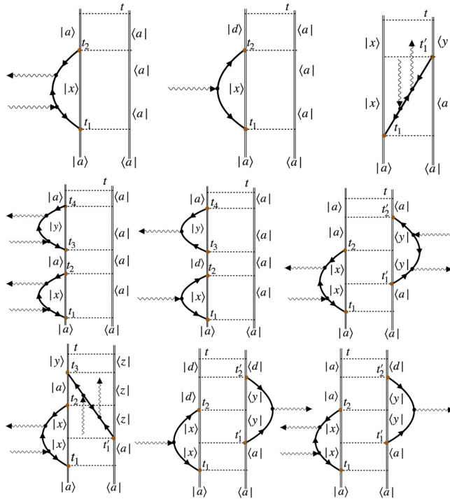
FIG. 3. Representative diagrams in the perturbation theory in the pump-field and (qubit) system-entangled field interactions. Top panel: second-order and lower panels: fourth-order interaction diagrams that contribute in time-evolution of the reduced system density matrix. States |a\rangle and |d\rangle denote the ground and doubly excited states |00\rangle and |11\rangle , respectively, and |x\rangle, |y\rangle, |z\rangle denote single-excited states |01\rangle and |10\rangle . Thick black lines are propagators for the entangled field where an arrow pointing toward (away) the vertex (brown dots) denotes field annihilation (creation) operator \hat{E}(\hat{E}^\dagger) . The field propagator is computed with respect to the effective action S_{\text{eff}}^0 (see the text). The whole set of diagrams can be obtained by considering propagators connecting to vertices not connected in the above diagrams.
