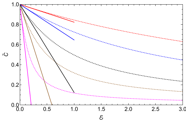
Fig. 1. Variation of the Concurrence with the pump pulse amplitude for spectral widths, \sigma_p = 0.1 (red), 0.2 (blue), 0.5 (black), 1.0 (brown), and 5.0 (magenta). Dashed curves are obtained from Eq. (2) using non-perturbative density-matrix elements from Eqs. (B12)–(B14), solid lines are the analytic result, Eq. (8), obtained using the perturbative results, Eqs. (3)–(6).
