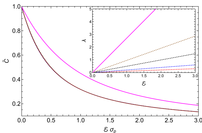
Fig. 2. Variations of the Concurrence with the scaled pump pulse amplitude \varepsilon\sigma_p for the same set of spectral widths as in Fig. 1. All curves for smaller \sigma_p < 5.0 (magenta) exhibit the scaling predicted by perturbative Eq. (8), even beyond the range of \varepsilon where \lambda > 1 and the perturbative expression is not valid, as shown in the Inset.
