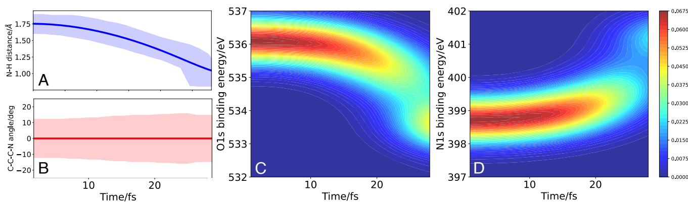
Fig. 4. ( A and B ) Time evolution of the average N–H distance and C–C–C–N dihedral angle calculated by the expectation value of wave packet. The corresponding wave packet widths represented by the full width at half maxima (FWHM) are also presented. ( C and D ) are TR-XPS signals for \tau = 1 fs probe pulses for the oxygen 1s ionization with mean photon energy 538 eV and the nitrogen 1s ionization 403 eV, respectively.
