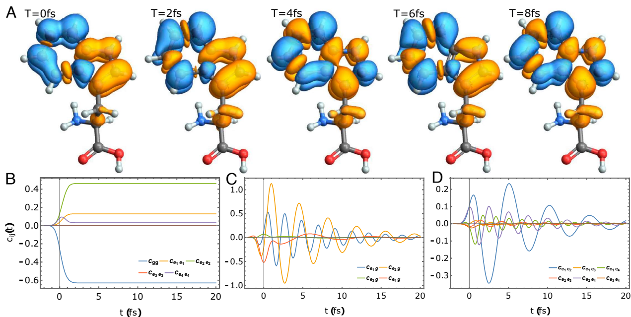
Fig. 9. Charge migration in L-tryptophan triggered by a Gaussian pump pulse E_p with central frequency \omega_p = 6 eV and spectral bandwidth \sigma_p = 0.9 eV. (A) Isosurfaces representing the difference charge density \langle \sigma(r, T) \rangle - \langle \sigma(r, 0) \rangle . (B–D) represent the time evolution coefficients of the populations c_{ee} , ground to valence coherence c_{eg} , and excited state contributions respectively; see Appendix 5.1.
