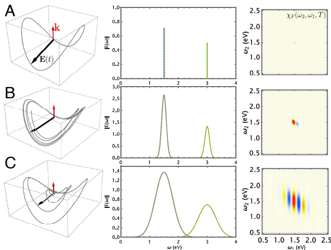
Fig. 2. Left: Light polarization trajectory in time domain. The red arrow represents the wavevector of the \mathbf{E}_1 and \mathbf{E}_2 fields, and the black arrow is the polarization of the total field. Center: Spectral envelopes used for the three field components used in the SFG process. Right: Corresponding chiral field correlation function, Eq. 11 with \omega = \omega_1 + \omega_2 . Three cases are considered: (A) Monochromatic fields, Eq. 8 ( E_\omega = 1 au, E_{2\omega} = 0.5 au, \omega = 1.5 eV, \theta = \pi/4 , \alpha_x = 0.2 , \alpha_y = \pi/2 , \phi = 0.6 ). (B) Narrowband fields centered at 1.5 eV (X,Y components) and 3 eV (Z component). (C) Broadband fields with the same central frequencies.
