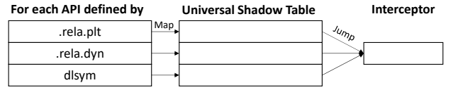
Figure 2: Overview of Universal Shadow Table.
