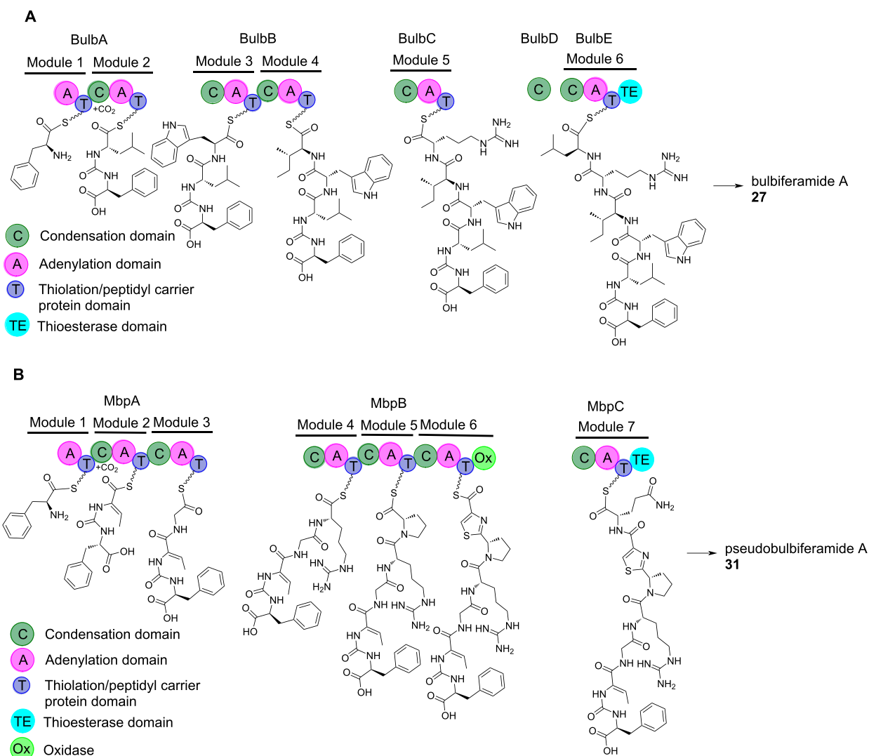
Figure 11: Proposed NRPS assembly lines for the biosynthesis of (A) bulbiferamide A ( 27 ) and (B) pseudobulbiferamide A ( 31 ).
