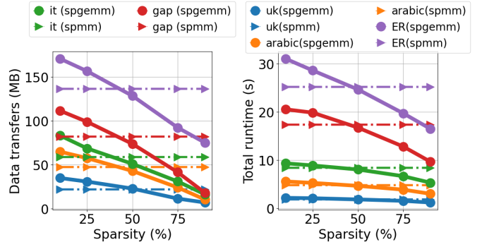
Fig. 7: The Figure shows the comparison results of the TS-SpGEMM and SpMM version. The left sub-figure shows the communication volume and the right sub-figure shows the runtime for different sparsity levels.
