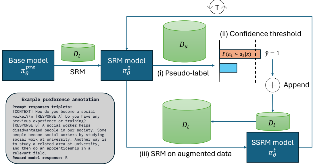
Figure 1: Semi-Supervised Reward Modeling (SSRM) enhances the ability of a language model to predict preferences using both labeled and unlabeled data. Given a pretrained model \pi_{\theta}^{pre} , a small labeled dataset D_l and a large unlabeled dataset D_u , we first perform supervised reward modeling (SRM) on D_l to obtain the SRM model \pi_{\theta}^0 . Then, at each step t , we perform three steps: (i) Pseudo-labeling: assign pseudo-labels to examples in D_u . (ii) Confidence thresholding: given a prompt x and two responses a_1, a_2 , if the prediction confidence exceeds a preset threshold, append it to the labeled dataset to obtain D_t . (iii) SRM on augmented data: finetune the model on D_t .
