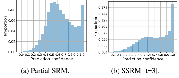
Figure 3: The prediction confidence noticeably improves on Gemma-2B models after three iterations of SSRM. Combined with better calibration, it shows the prediction more accurately reflects the actual outcome.
