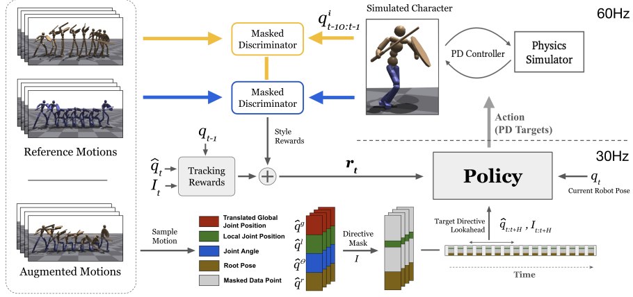
Fig. 3: Illustrates the architecture and training details of the MHC framework, which consists of a controller and an ensemble of discriminators. Here the controller is trained to follow an augmented set of masked directives derived from the provided MoCap dataset. The controller gets feedback via tracking objective and style rewards generated by the ensemble of discriminators. Together they enable a directable policy to generate physically realistic motions capable of catching up, combining primitives, and completing motions from under-specified directives.
