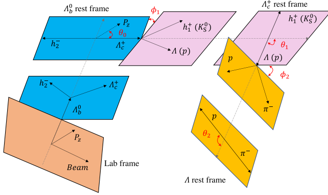
FIG. 2. Definition of the helicity angles for \Lambda_b^0 \rightarrow (\Lambda_c^+ \rightarrow \Lambda h_1^+) h_2^- and \Lambda_b^0 \rightarrow (\Lambda_c^+ \rightarrow p K_S^0) h^- decays, where h_1^+ , h_2^- denote the kaon or pion.
