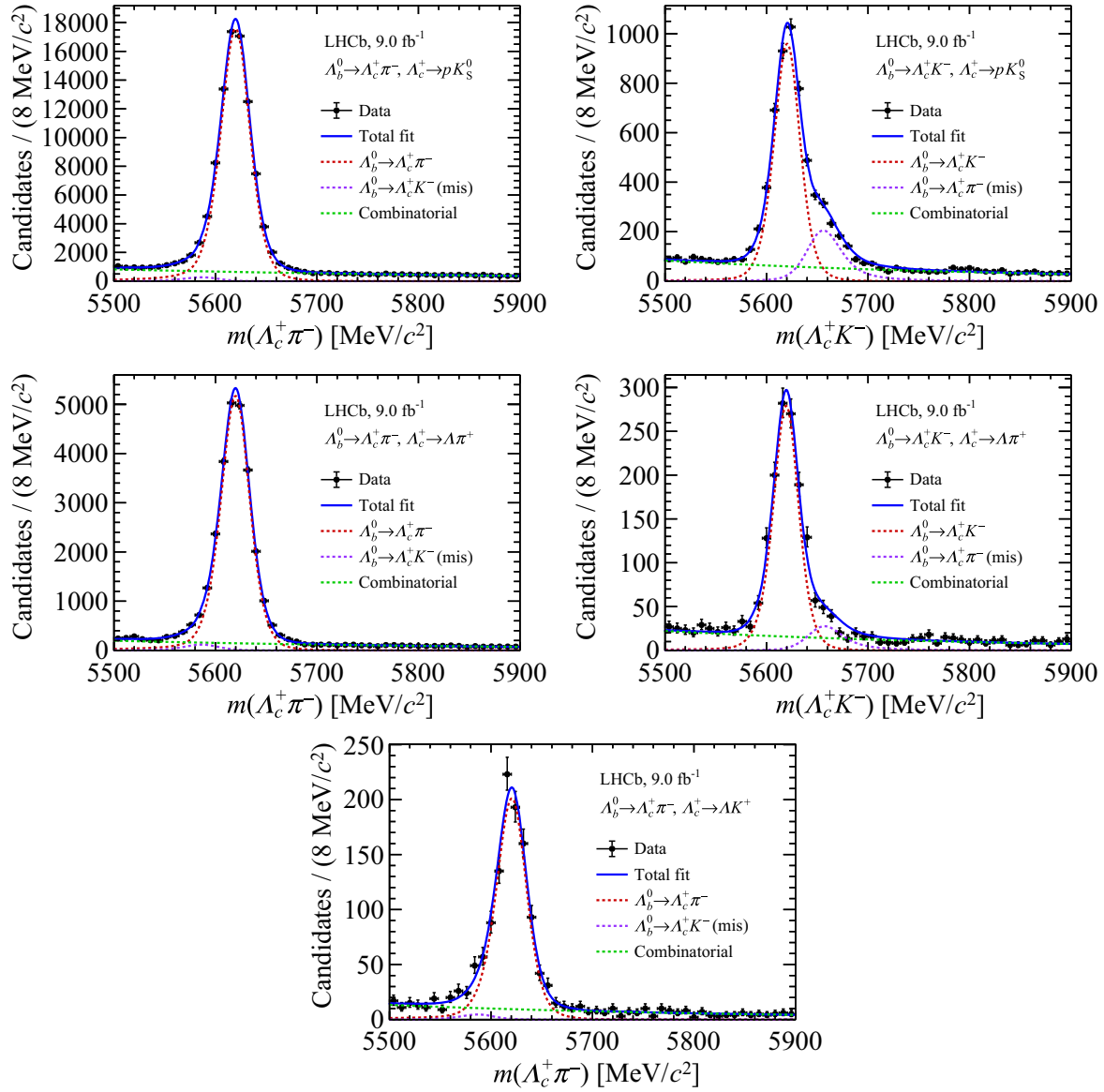
FIG. 1. The invariant-mass distributions of \Lambda_b^0 candidates reconstructed in the (top left) \Lambda_b^0 \rightarrow \Lambda_c^+(\rightarrow p K_S^0)\pi^- , (top right) \Lambda_b^0 \rightarrow \Lambda_c^+(\rightarrow p K_S^0)K^- , (middle left) \Lambda_b^0 \rightarrow \Lambda_c^+(\rightarrow \Lambda\pi^+)\pi^- , (middle right) \Lambda_b^0 \rightarrow \Lambda_c^+(\rightarrow \Lambda\pi^+)K^- , and (bottom) \Lambda_b^0 \rightarrow \Lambda_c^+(\rightarrow \Lambda K^+)\pi^- decays, with the fit results drawn.
