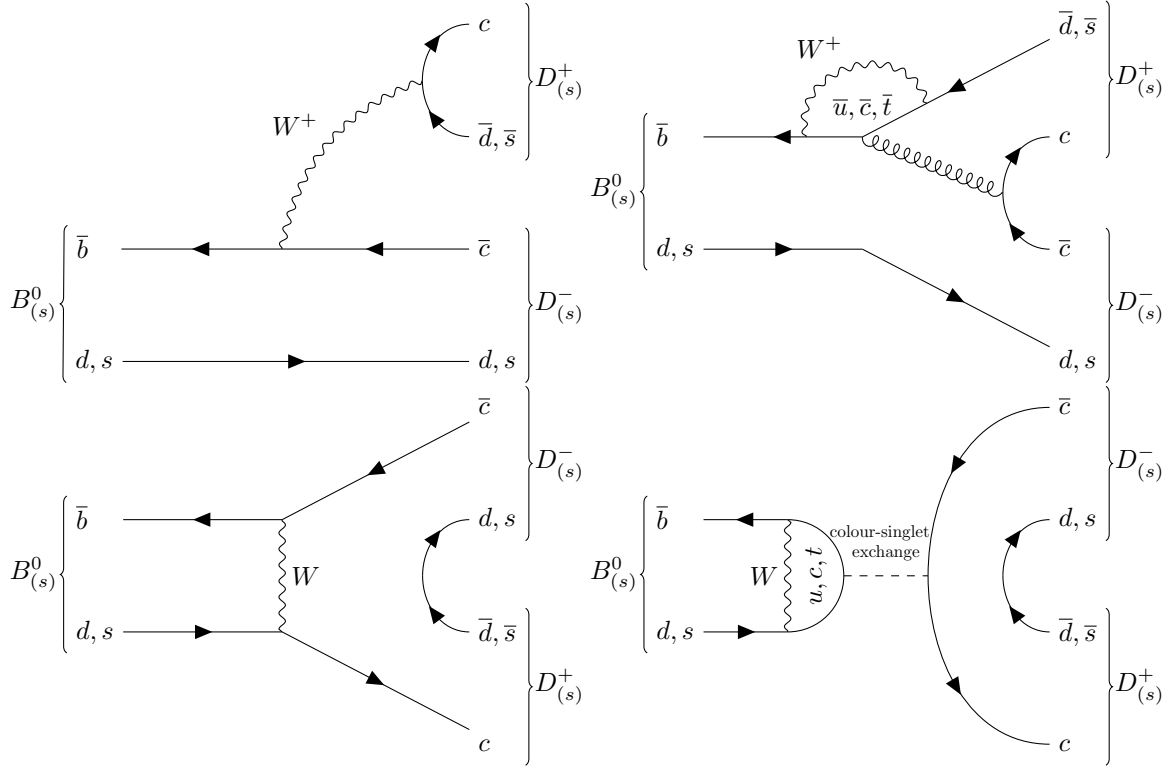
Figure 1. Dominant Feynman diagrams contributing to the B^0 \rightarrow D^+ D^- and B_s^0 \rightarrow D_s^+ D_s^- decays. The (top left) tree-level, (bottom left) exchange, (top right) penguin and (bottom right) penguin annihilation diagrams are shown.
