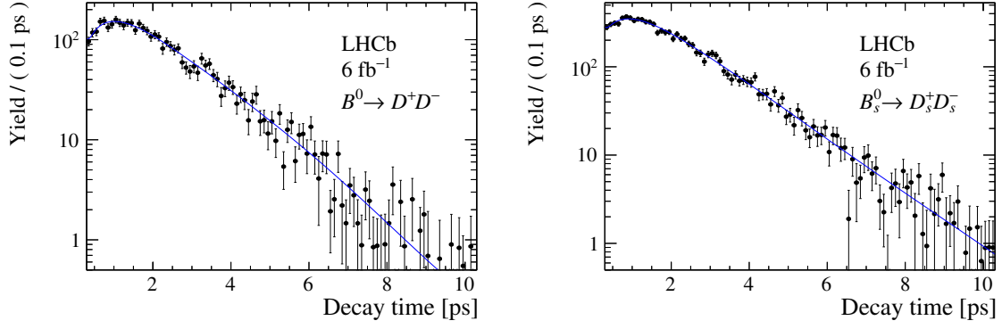
Figure 4. Decay-time distribution of (left) B^0 \rightarrow D^+ D^- and (right) B_s^0 \rightarrow D_s^+ D_s^- candidates. The background-subtracted data are shown as points and the projection of the PDF is shown as a solid blue line.
