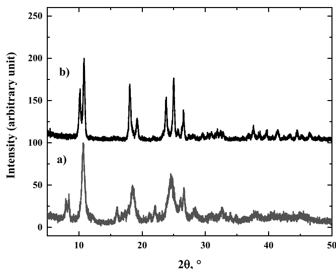
Figure 4. The x-ray diffraction patterns for [\text{Fe}(\text{Htrz})_2(\text{trz})](\text{BF}_4) (a) nanoparticles, and (b) nanorods.
