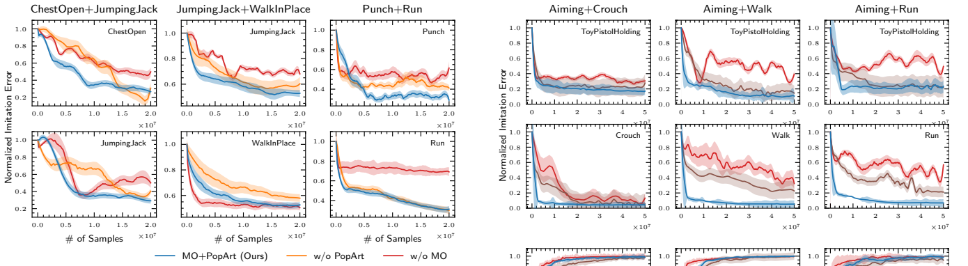
Fig. 10. Learning performance on tasks of composite motion learning from two single-clip reference motions, which are illustrated in Fig. 4. "MO" stands for the proposed multi-objective learning framework detailed in Section 4.3. Colored regions denote mean values \pm a standard deviation based on 10 trials.
