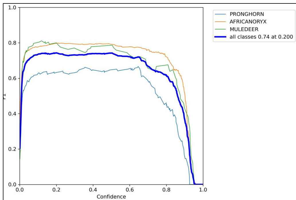
Figure 10 F1 curve provides insights into the overall detection performance of the mode at different confidence thresholds, enabling model selection, optimization, and comparison across different experiments or variations of the algorithm.
