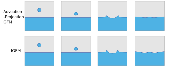
Fig. 10. Comparison experiment: A liquid drop falling into a tank. Top: Advection-Projection GFM. Bottom: IGFM.
