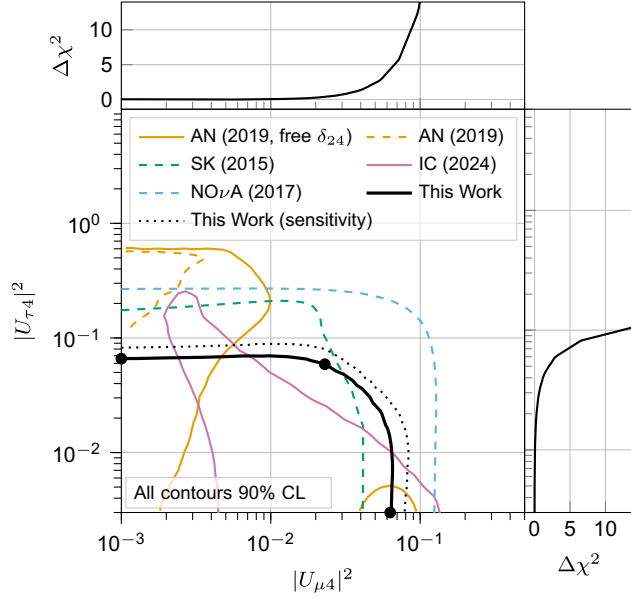
FIG. 5. Contour of the 90% CL limit of this analysis compared to measurements from the ANTARES [32], Super-Kamiokande [45] and NOνA [14] experiments and a recent high-energy IceCube oscillation study [46]. Black dots along the contour of this work indicate where coverage spot-checks were run. The dotted line shows the expected sensitivity of this analysis. Results shown as dashed lines assume \delta_{24} = 0 .
