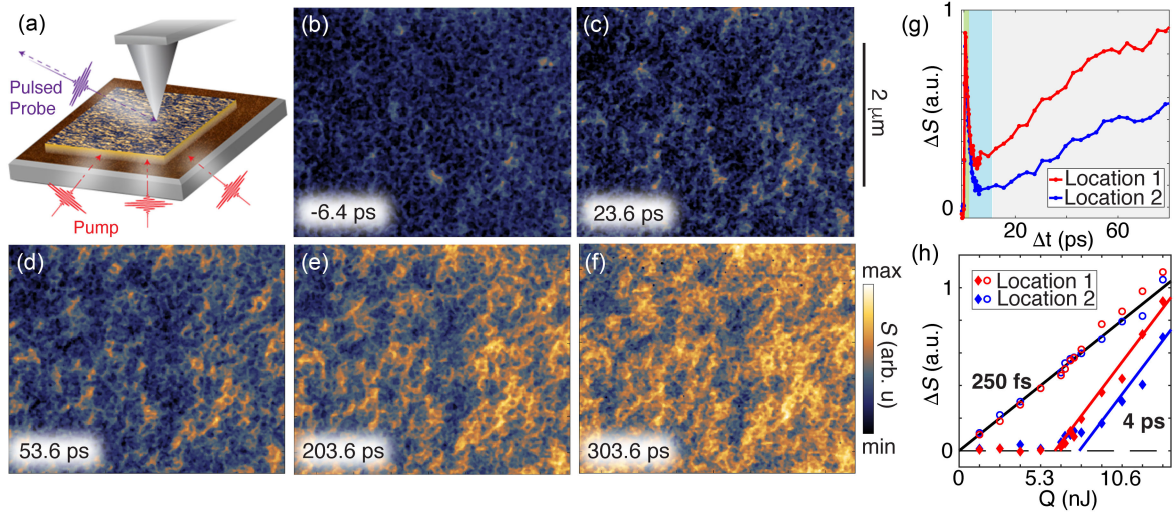
FIG. 1. Nano-optical study of the light induced IMT in a \text{VO}_2 film. All data in Fig. 1 were obtained with an initial temperature T_i = 330 K. (a) Schematic of the experiment. A horizontally polarized pump beam (red pulses) initiates the IMT. We use a vertically polarized 8\ \mu\text{m} wavelength pulsed probe (purple pulse) focused on an AFM tip to monitor the local near-field amplitude, S , at a variable time delay, \Delta t , after photoexcitation. In our experiments, temperature dependent data is obtained by changing the initial (equilibrium) temperature of the sample, T_i , with a heat stage. (b)–(f), Images of S , using 5.3 nJ of photoexcitation power, obtained (b), before photoexcitation: \Delta t = -6.4 ps, and (c)–(f), after photoexcitation: (c) \Delta t = 23.6 , (d) \Delta t = 53.6 , (e) \Delta t = 203.6 , (f) \Delta t = 303.6 ps. (g) Dynamics of the pump induced change of the near-field amplitude \Delta S obtained at two representative locations, Location 1 and location 2, where values of S are near the extremes of high and low contrast observed in panel (f), respectively. The green, blue, and gray shaded regions mark the first, second, and third stages, respectively, of the three-step response to photoexcitation as described in the main text. (h) Data of \Delta S are shown against the photoexcitation energy at the same two locations investigated in panel (g). Data collected at \Delta t = 250 fs are shown with open circles, while data obtained at \Delta t = 4 ps are shown with filled diamonds. Note that systematic inhomogeneity observed at \Delta t = 250 fs and above Q_c likely derives from carriers that have abruptly transitioned to the metallic state (see Supplemental Material [19], Sec. 2.4 for details and discussion).
