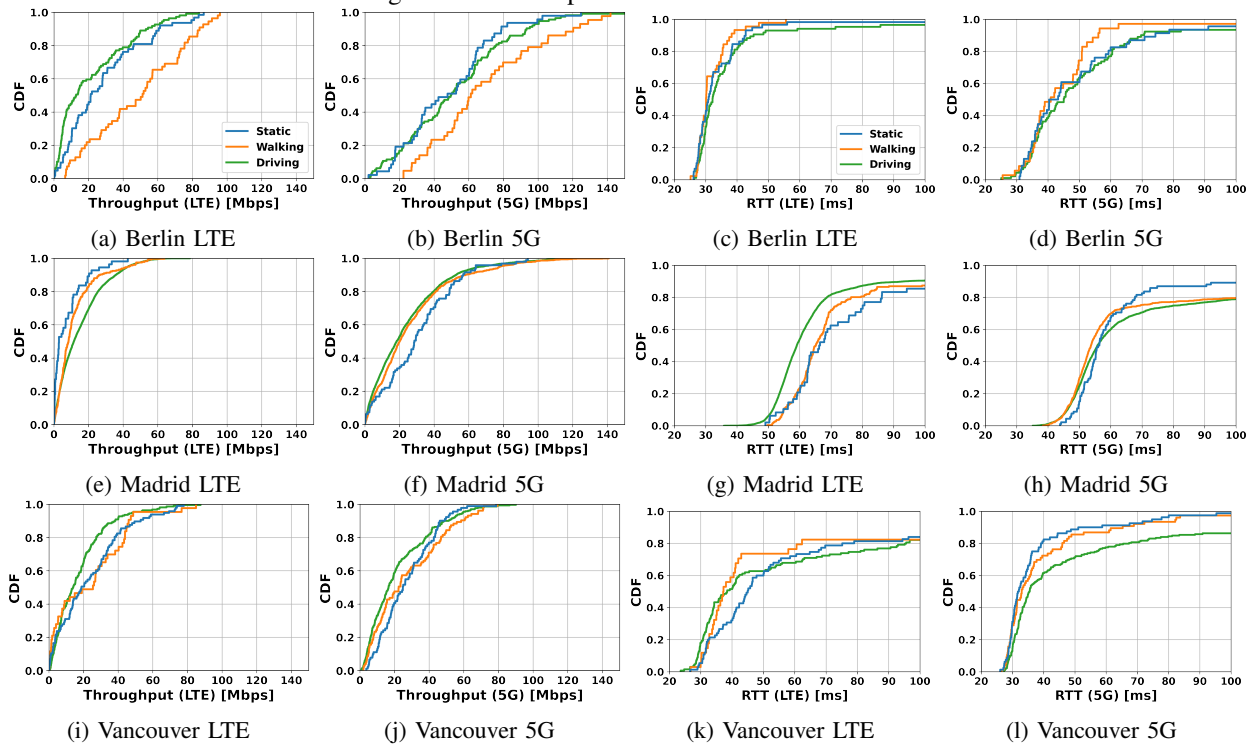
Fig. 7: Throughput &amp; Latency Comparison across different mobility modes.
