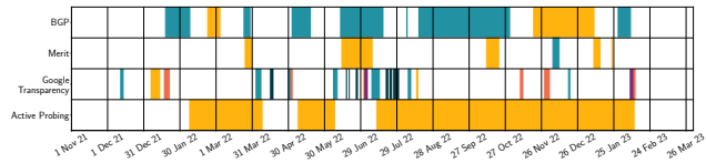
(f) Pakistan IODA Signals
