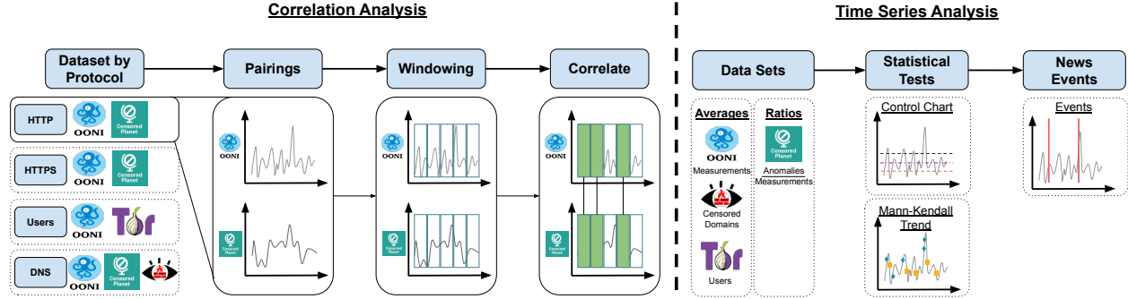
Fig. 1: The pipeline for the methodology of our correlation analysis and our time series analysis. In the correlation analysis, we take pairs of datasets by protocol, window the datasets, and then run Spearman's rank and Kendall rank correlations. In the time series analysis, we run the control chart and Mann-Kendall trend detection tests on the various datasets. Then, we collect the news articles to identify plausible censorship-causing events.
