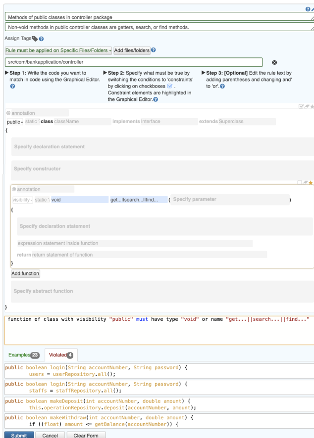
Figure 3: A developer using RulePad creates design decisions by specifying properties and refining rules in the Graphical Editor (top) with structured code snippets. They can verify and optionally edit rules in the Textual Editor (bottom) while viewing examples of code that satisfy or violate the rule.
