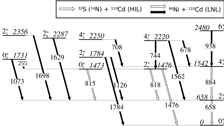
Fig. 4. Partial level scheme of ^{110}\text{Cd} presenting the \gamma -ray transitions observed in the ^{60}\text{Ni} + ^{110}\text{Cd} experiment with their energies given in keV. The transitions marked in black were only observed in the experiment using ^{60}\text{Ni} beam, while the transitions marked in white were observed in all three Coulomb-excitation experiments, i.e. with ^{14}\text{N} , ^{32}\text{S} , and ^{60}\text{Ni} beams. Only states assigned in Refs. [8, 9] to the ground-state band, the bands built on the 0_{2,3}^+ states, and the K = 2 ‘ \gamma ’ and ‘ \gamma -intruder’ bands are plotted.
