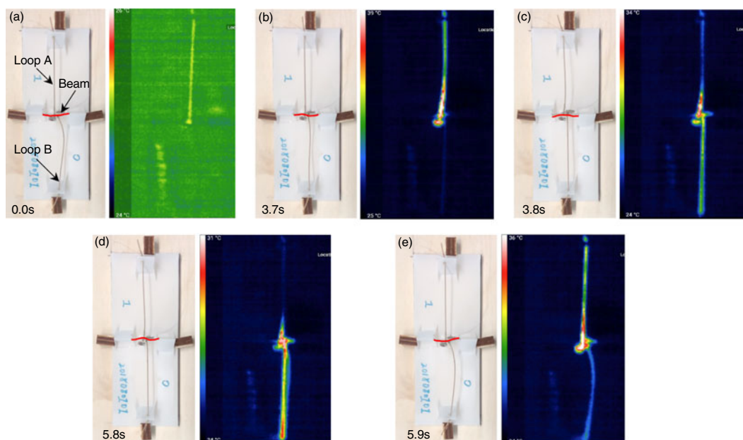
Fig. 8. The first oscillation cycle of the foldable oscillator. In each figure from (a) to (e), the left side is the image of the oscillator and the right side is the corresponding thermal image obtained with a thermal camera. The red lines in the figures indicate the contours of the bistable beam in different states.
