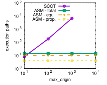
Fig. 6. The number of branches of (total = prove equivalent + prove property alone) is several orders of magnitude shorter than SCCT. SCCT is unbounded (increases exponentially).
