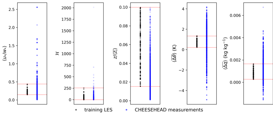
Fig. 7 Distribution of the predicting variables ( \langle u_*/w_* \rangle , \mathcal{H} , z/z_i , \langle \Delta \theta \rangle , \langle \Delta q \rangle ) used for the model training (gray) and of the predicting variables that occur in the CHEESEHEAD19 field measurements (blue). The limits of the predictor variables used for training the model are shown by the red dotted lines
