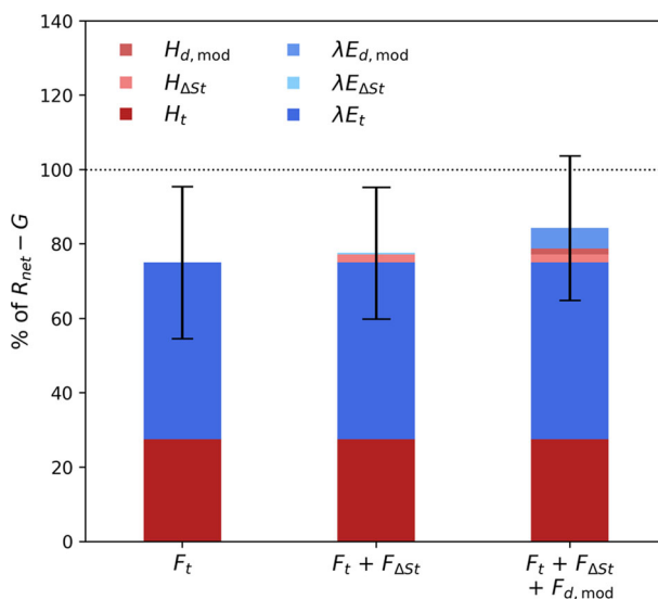
Fig. 9 Share of turbulent heat fluxes ( H_t , \lambda E_t ), air storage change ( H_{\Delta St} , \lambda E_{\Delta St} ) and modelled dispersive heat fluxes ( H_{d,\text{mod}} , \lambda E_{d,\text{mod}} ) of the total available energy ( R_{\text{net}} - G ). The error bars represent the standard deviation of the sums shown in each bar
