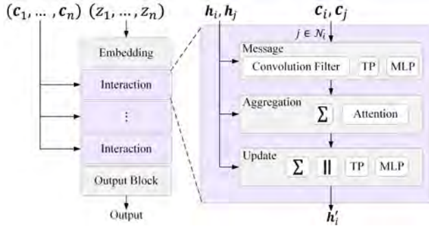
Fig. 20. A general architecture of higher order equivariant models. Each model consists of several interaction blocks which perform pairwise message passing between atoms. Here, \Sigma denotes summation, \parallel denotes feature concatenation, TP refers to the Tensor Product of feature vectors, and MLP refers to multilayer perceptrons. The specific operations used in each Message, Aggregation, and Update blocks differ between models, but existing methods such as TFN [Thomas et al. 2018], NequIP [Batzner et al. 2022], SE(3) -Transformer [Fuchs et al. 2020], Equiformer [Liao and Smidt 2023], Cormorant [Anderson et al. 2019], and SEGNN [Brandstetter et al. 2022a] all fall under this framework.
