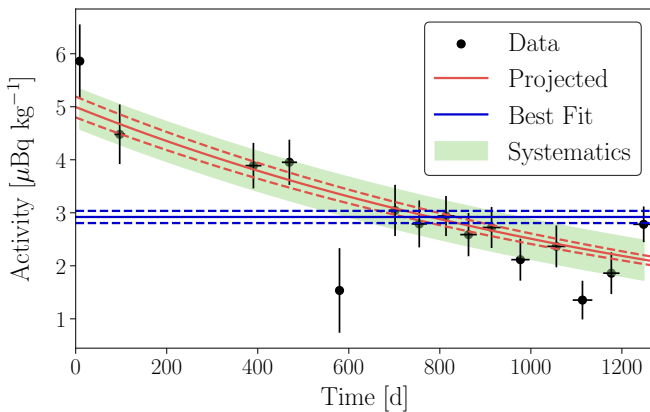
FIG. 5. Activity of ^{125}\text{Sb} in the Crystals volume extracted from the individual-dataset fits (black dots). The blue lines (solid and dashed) depict the mode and the statistical uncertainty of the activity from the best fit, where all the dataset are grouped together. The red line is the projected time-dependent activity, computed by assuming the best fit to be the integral average along time of a decaying activity with the tabulated half-life of 2.76 yr. The green band shows the systematic uncertainty coming from the comparison between each individual-dataset fit and the time-dependent activity obtained by the reference fit.
