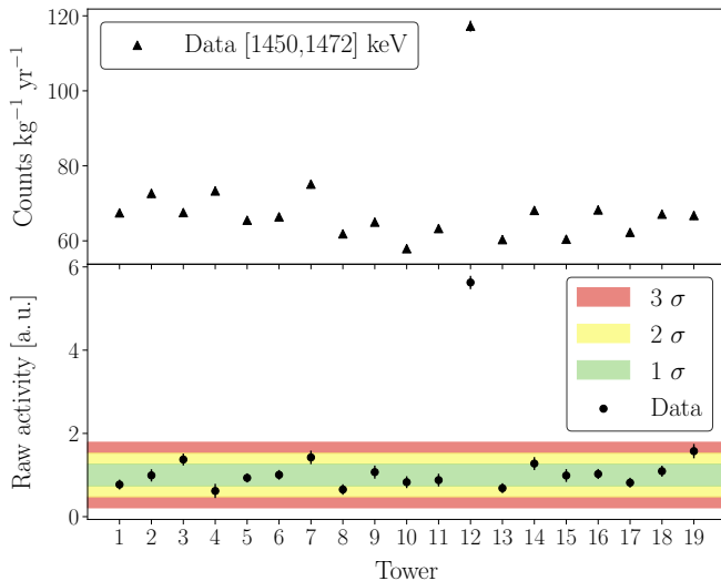
FIG. 7. (Top) Yield normalized by the exposure for the potassium 1461-keV line of ^{40}\text{K} for the 19 towers of CUORE. Tower 12 contains approximately double the events compared to the other towers. (Bottom) Normalization factor of the ^{40}\text{K} contamination in the Crystals bulk when performing the fit on the towers individually. The colored bands refer to the 1, 2 and 3 standard deviations coming from the activity distribution when considering all the towers except tower 12.
