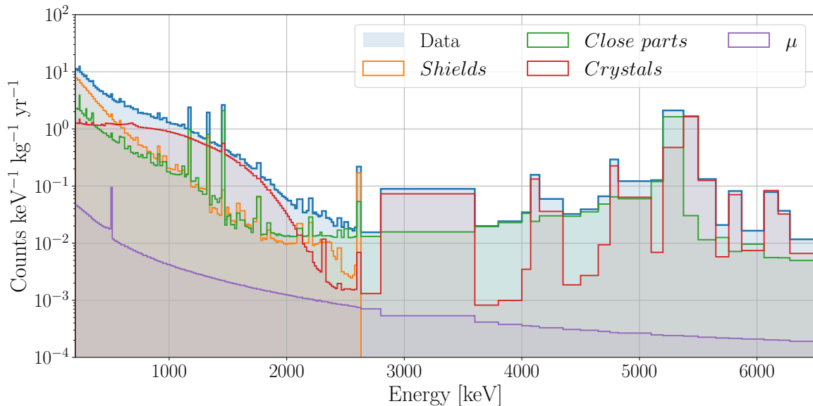
FIG. 4. Decomposition of the CUORE data by source location. The Shields group includes the volumes ELS , Outer shields , TL , ILS and Inner shields .
