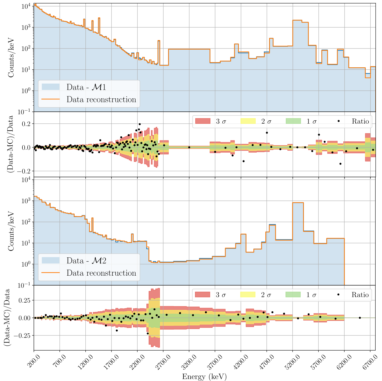
FIG. 3. ( Top panels ) Reconstruction of the \mathcal{M}1 events and residuals. ( Bottom panels ) Cumulative spectrum of the individual \mathcal{M}2 events and residuals. The residuals are quoted as fractions of data, with the statistical uncertainties represented as 1\sigma , 2\sigma and 3\sigma standard-deviation bands. The \mathcal{M}2 spectrum ends at 6200 keV because this is the maximum energy for the events in the highest total-energy band taken into account.
