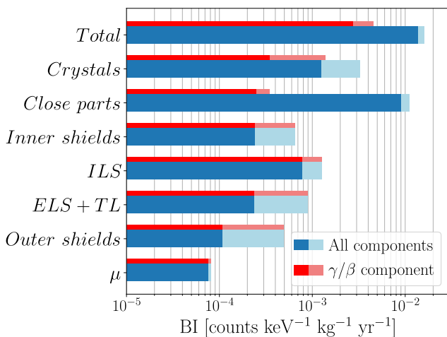
FIG. 6. BI components obtained from the full set of fits used to extract the systematic uncertainty. The light (dark) blue band represent the 16% (84%) quantile of the BI distribution obtained. The red bands indicate the corresponding fraction due to \beta and \gamma events.
