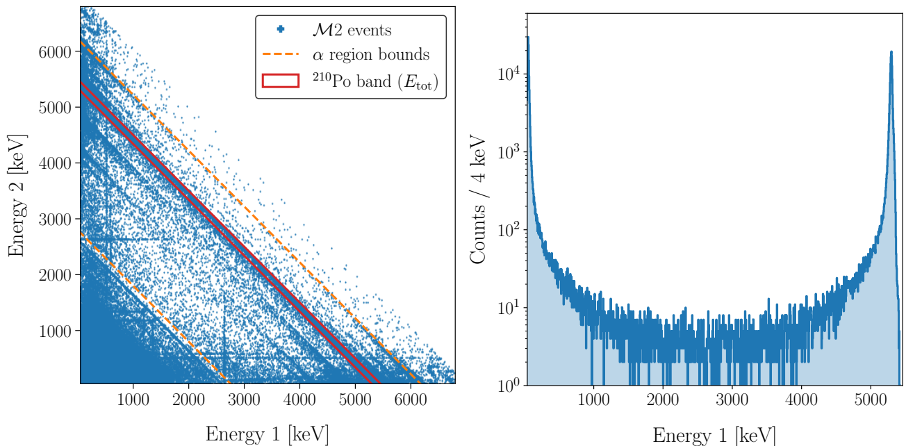
FIG. 2. ( Left ) Individual energy depositions in \mathcal{M}2 data. The diagonal bands represent events with a constant total-energy shared between the two detectors involved. As an example, the region enclosed by the solid red line corresponds to total energies around the decay of ^{210}\text{Po} at 5.4 MeV (summing to the \alpha energy and to the Q-value). The vertical and horizontal bands correspond to full-energy photo-peaks, where almost the totality of the \gamma -ray energy is registered by one of the two detectors involved in the \mathcal{M}2 event. ( Right ) Projection of the ^{210}\text{Po} -decays for \mathcal{M}2 events (region inside the solid red line) onto the x-axis. The peaks at \sim 100 keV \sim 5300 keV are due to the cases of \alpha particle and a recoiling nucleus detected in two different crystals; the region in-between is populated by events where the \alpha particle deposits a fraction of its energy in both crystals.
