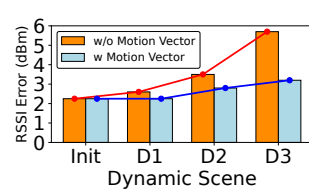
Figure 14: Impact of Scene Dynamics
