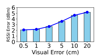
Figure 16: Visual Prior Sensitivity Analysis
