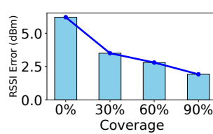
Figure 15: Impact of Camera Coverage
