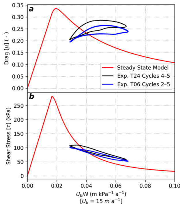
Figure 9. Comparison of (a) drag and (b) shear stress responses as a function of effective pressure normalized slip velocity ( U_b/N ) for steady-state model predictions (red) and observed values from exp. T24 (black) and Exp. T06 (blue) during cycles with stable mean cavity geometries (cycle numbers in key; also see Figs 3 and 5–8). All estimates shown use U_b = 15 \text{ m a}^{-1} .
