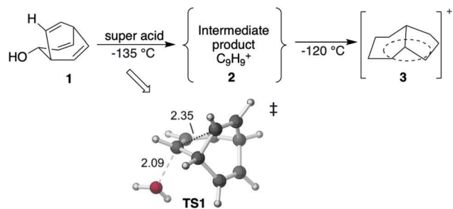
Scheme 1 Previous experiments on C_9H_9^+ cations. 50 The transition state TS1 is visualized using CYLVIEW 1.0, 51 with key bond lengths labeled in Å. The C–O bond breaks first, and the C–C bond formation occurs subsequently in an asynchronous manner (see ESI† for details).
