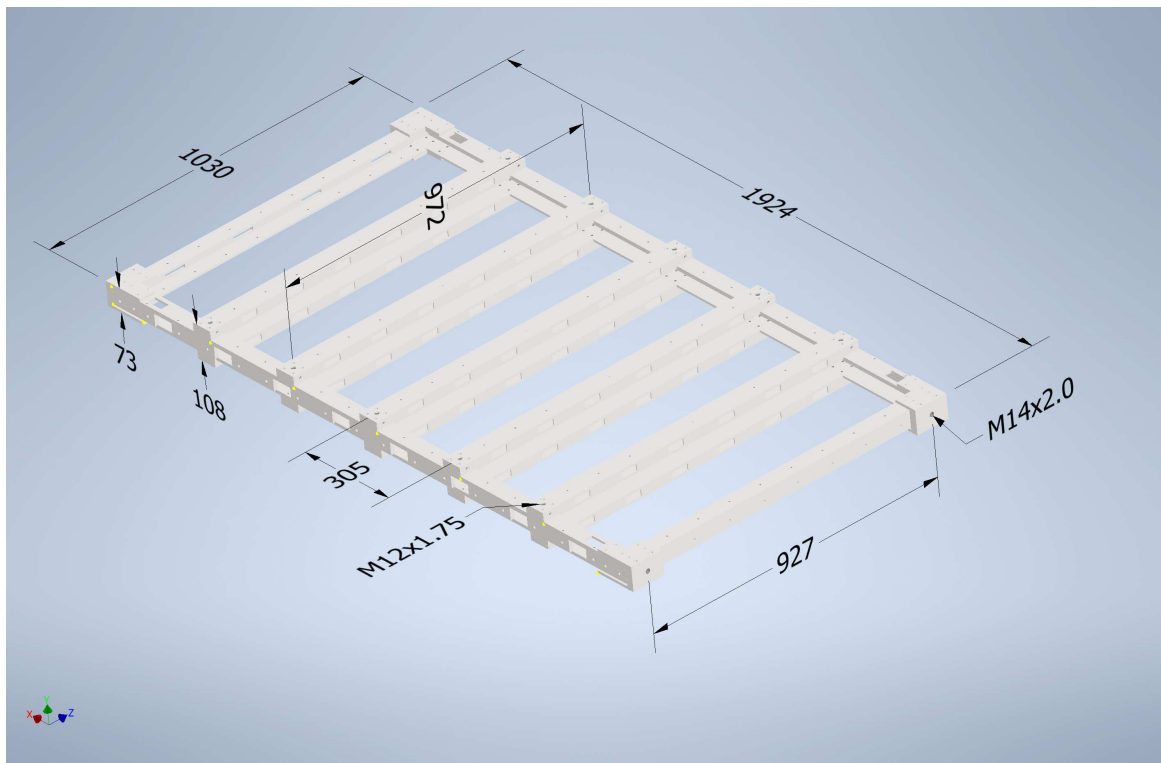
Figure 11. CX1 module frame for CODEX- \beta with dimensions in mm. Relevant pick points are also indicated.
