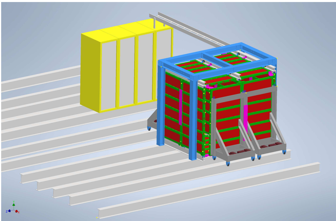
Figure 15. Diagram of CODEX- \beta in the D1 barrack with needed services racks and proposed cable tray. The floor panels of the D1 barrack are not shown, but the structural support beams are.
