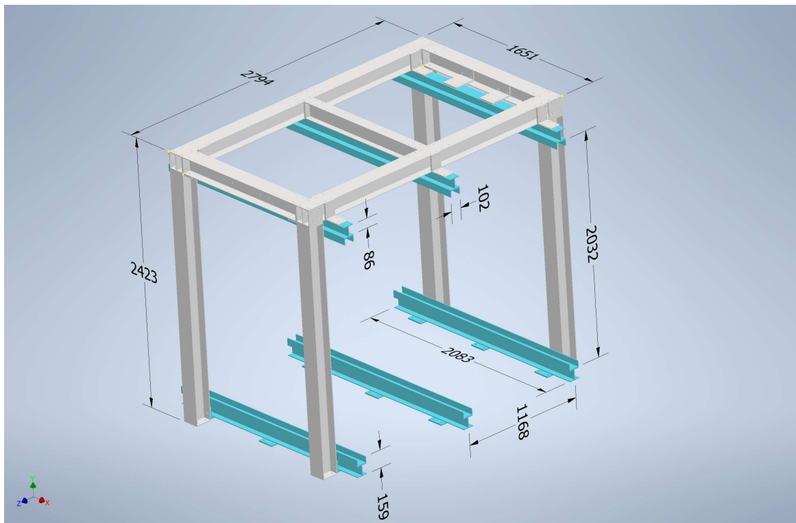
Figure 12. CODEX- \beta support structure with dimensions in mm.
