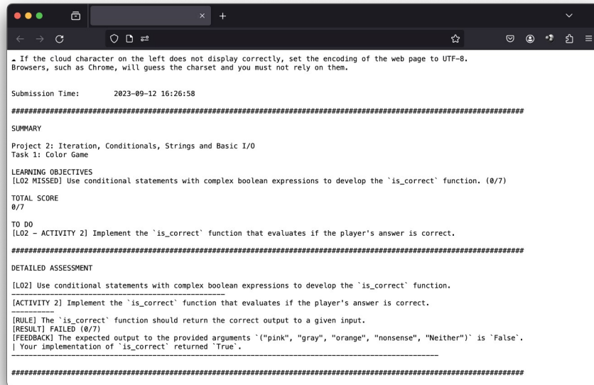
Fig. 2. The feedback shown to students for a submission that contains an incorrect solution.
