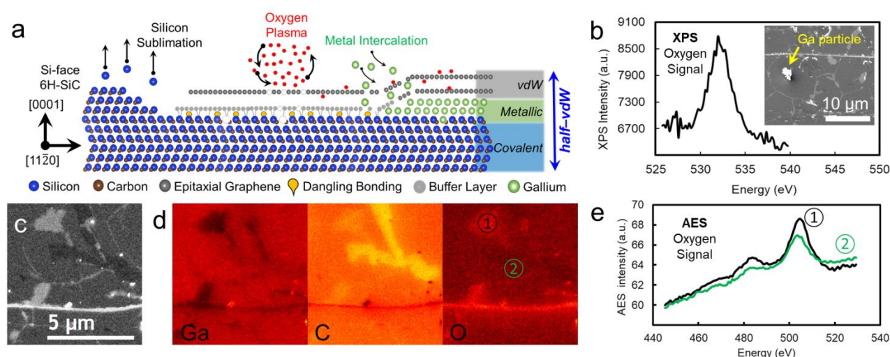
Figure 1. Presence of oxygen signal in 2D gallium-intercalated epitaxial graphene. (a) a schematic represents the fabrication steps of Ga interaction of a monolayer epitaxial graphene. The buffer layer is detached and forms a bilayer graphene cap over a bilayer Ga layer. The final structure is called half-vdW heterostructure because it achieves three bonding types across the interface. (b) XPS signal from 2D-Ga surface. The insert is an SEM image shows a micrometer-size oxidized Ga particle in the surface which could contribute to the XPS oxygen signal. (c) Higher magnification SEM image and (d) the corresponding auger electron spectroscopy (AES) maps for gallium, carbon, and oxygen. (e) AES point spectrum at the oxygen signals from sites 1 and 2 as indicated in the oxygen map in (d). The AES maps and the signal spectrum from site 2 confirm that there is oxygen co-located with the gallium. However, the plane-view AES characterization cannot confirm if the 2D-Ga layer is oxidized.
