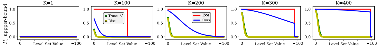
Fig. 3. Probability that the system is unsafe: our bound from Cor. 1 (blue), ISSf bound (red). The x-axis is the level set expansion -\epsilon and the y-axis is the failure probability (lower is better). The plots from left to right indicate safety for K = 1, 100, 200, 300 , and 400 steps. Simulations where \mathbb{E}[h(\mathbf{x}_k) | \mathcal{F}_{k-1}] = \alpha h(\mathbf{x}_k) and approximate probabilities from 1000 samples are shown for simulations where h(\mathbf{x}_k) is sampled from 3 different conditional distributions: uniform (pink), truncated Gaussian (green), and a categorical (yellow) all which satisfy Cor. 1.
