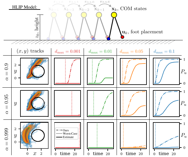
Fig. 1. Safety results for a bipedal robot navigating around an obstacle. Details are provided in Section IV. (Top) Visualization of the Hybrid Linear Inverted Pendulum (HLIP) model. Yellow indicates the center-of-mass (COM), blue is the stance foot, and red is the swing foot. The states x_k are the global COM position, the relative COM position, and COM velocity, and the input is the relative position of the feet at impact. (Bottom) A table with variable maximum disturbance value ( d_{\max} ) and controller parameter ( \alpha ) shows our (dashed lines) theoretical bound on safety failure from Thm. 3, (dotted lines) the shortest first-violation time based on the worst-case disturbance approximation, and (solid lines) approximated probabilities from 5000 trials (lower is safer). On the left, the trajectories of the COM are shown walking from bottom left towards the top right while avoiding the obstacle with each color corresponding to a different d_{\max} . The robot attempts to avoid the obstacle (black).
