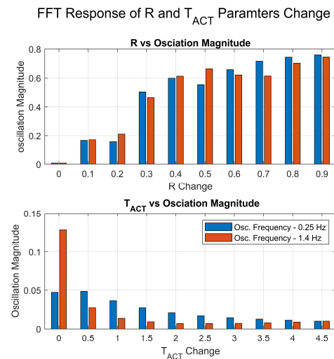
Figure 23. FFT response of R and T_{act} parameters' change.
