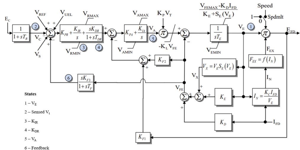
Figure 5. Block diagram of AC7B exciter model [36].
