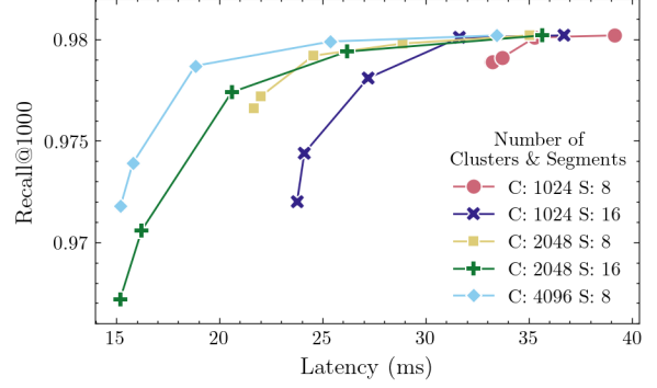
Figure 6: Recall vs. latency of ASC ( \eta=1 ) for varying values of \mu at retrieval depth k = 1000 . For each fixed number of clusters and segments, \mu varies from 0.4, 0.5, 0.6, 0.7, to 1.
