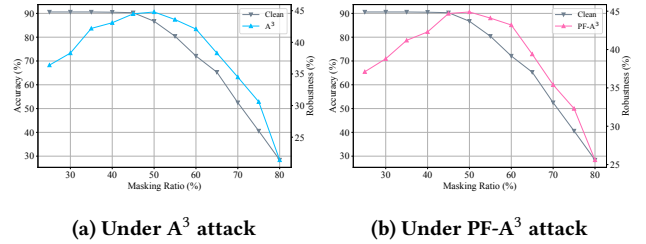
Figure 6: Illustration of how different masking ratios in the finetuning affect the performance.
