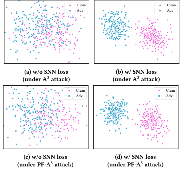
Figure 7: t-SNE visualization on CIFAR-10 by using our detector with/without SNN loss. For each experiment, we perform t-SNE visualization on 200 clean images and 200 adversarial examples generated either by the A 3 attack, i.e. , (a) and (b), or by the PF-A 3 attack, i.e. , (c) and (d).
