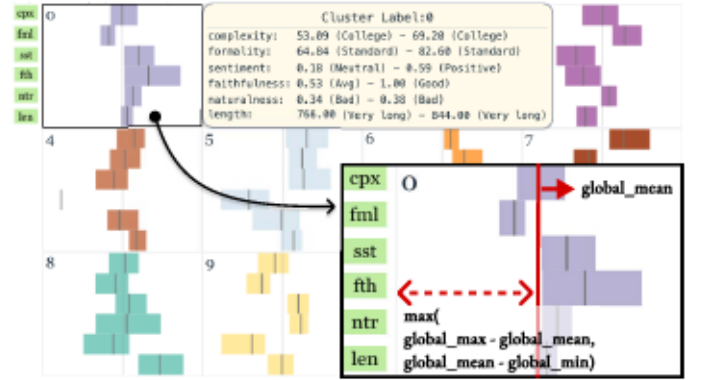
Fig. 5: Cluster Profiles visualize the feature ranges of each cluster with a scaled vertical bar chart. Each cluster is encoded by a unique color. The bars are aligned by the center vertical line, which encodes the global mean. The half of the profile width is encoded by \max(global\_max - global\_mean, global\_mean - global\_min) . This way, the bars are scaled to show the distinctiveness of each cluster. Hovering over a bar chart shows the ranges in values and categorization.
