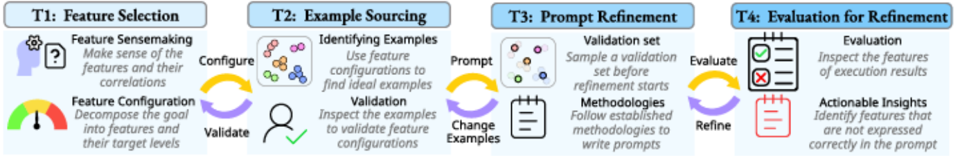
Fig. 2: The feature-oriented workflow for a systematic dataset-scale prompt evaluation. T1: Feature Selection. Designers should make sense of potential features to use for evaluation and their correlations, and then select a feature configuration that consists of a subset of features and corresponding target ranges. T2: Example Sourcing. Designers should use the feature configuration to find ideal examples, which are used to validate (and refine) the configuration and in the prompt. T3: Prompt Refinement. First, select a validation set before the refinement starts, and then follow established prompting methodologies to write the prompt that expresses the feature configurations. Execute the prompt for validation when ready. T4: Evaluation for Refinement. Inspect the evaluation result on selected features, identify cases that do not fit the feature configuration, and refine the prompt accordingly. We emphasize that features should be used as guidance, not targets.
