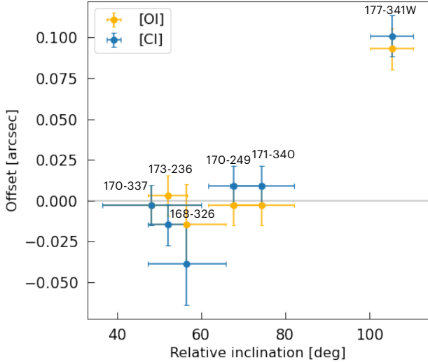
Fig. 4. Offsets between the intensity peaks of forbidden line emission and the location of the star, versus relative inclination. A relative inclination of 0 deg would correspond to a disk being irradiated face-on, and of about 90 deg to an edge-on configuration. The peak in the radial cut of [O I] 6300 Å is marked in yellow, and blue points mark the offset of [C I] 8727 Å.
