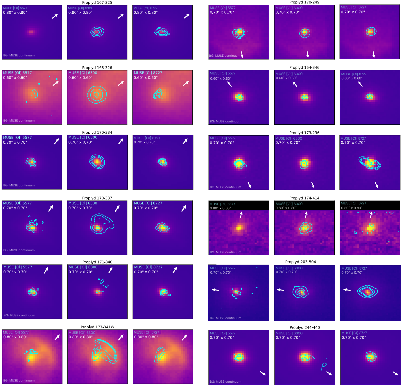
Fig. 2. Spatial comparison between MUSE stellar continuum (colormap) and MUSE emission lines (contours) for proplyds 154–346, 167–325, 168–326, 170–249, 170–334, 170–337, 171–340, 173–236, 174–414, 177–341W, 203–504, and 244–440. The emission line and the size of each image are shown in the top left corner. The contours represent 50%, 70%, and 90% of the peak intensity of the MUSE emission lines, except for the [C I] line of 174–414 for which only 90% is shown. The direction of the UV source is shown with an arrow.
