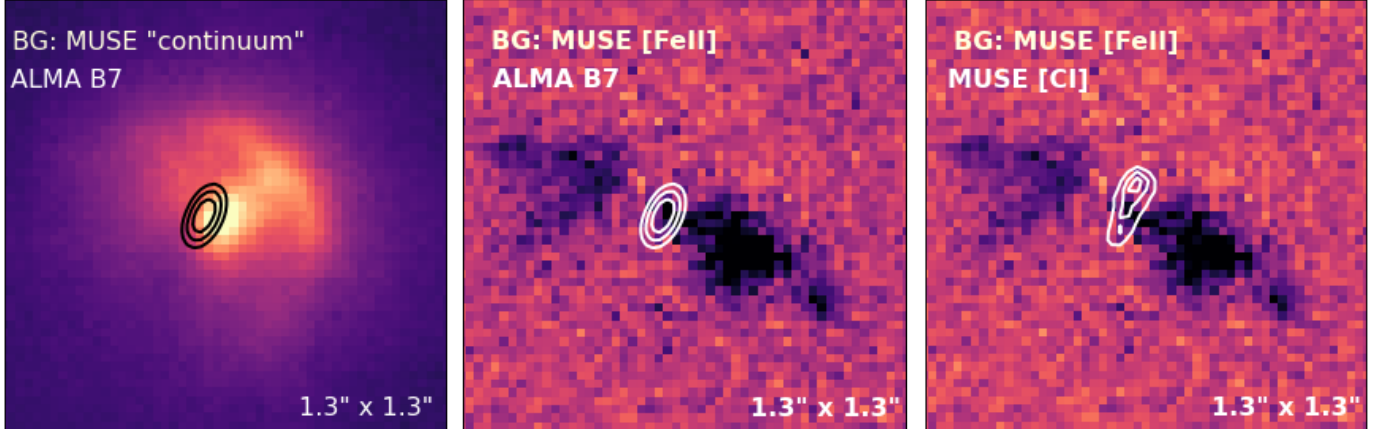
Fig. A.1. Proplyd 177-341W shown for three cases: 1) the stellar continuum emission in the background, overlaid with the contours of ALMA Band 7 data; 2) [Fe II] 8892 Å (MUSE) in the background, overlaid with the contours of ALMA Band 7 data; 3) [Fe II] 8892 Å (MUSE) in the background, overlaid with the contours of [C I] 8727 (MUSE).
