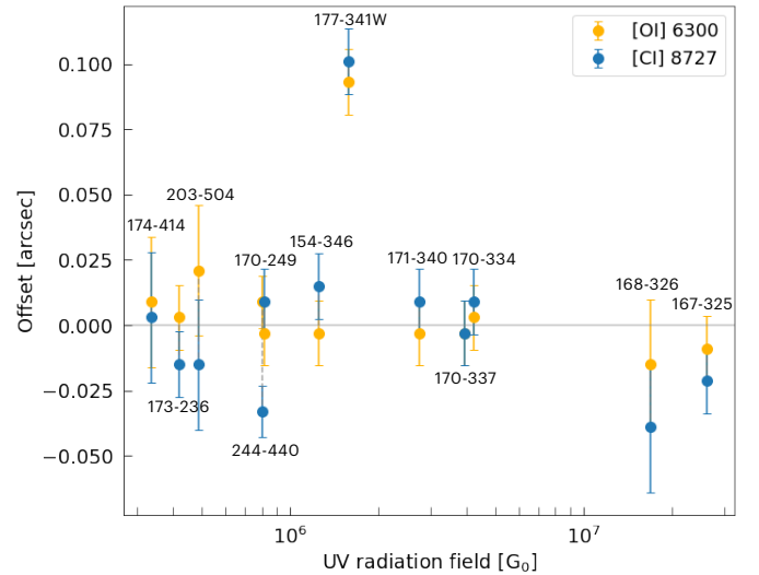
Fig. 3. Offsets between the intensity peaks of forbidden line emission and the location of the star versus the UV radiation field. The peak in the radial cut of [O I] 6300 Å is marked in orange, and blue points mark [C I] 8727 Å.
