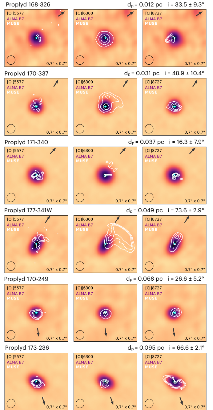
Fig. 1. ALMA Band 7 images of proplyds 168–326, 170–337, 171–340, 177–341W, 170–249, and 173–236 compared with the MUSE emission lines (contours) at 50%, 70%, and 90% of the peak intensity; the rows are ordered in increasing projected distance from \theta^1 Ori C. The ALMA Band 7 data were originally published by Eisner et al. (2018); the values for inclination marked above the figures are from Ballering et al. (2023), except for 168–326 and 171–340 (Ballering et al., in prep.). The MUSE emission lines are shown in the top left corner, the beam size is indicated in the bottom left corner, and the size of each image in the bottom right corner. The direction of the UV source is shown with an arrow. The cyan star marks the star's estimated location.
