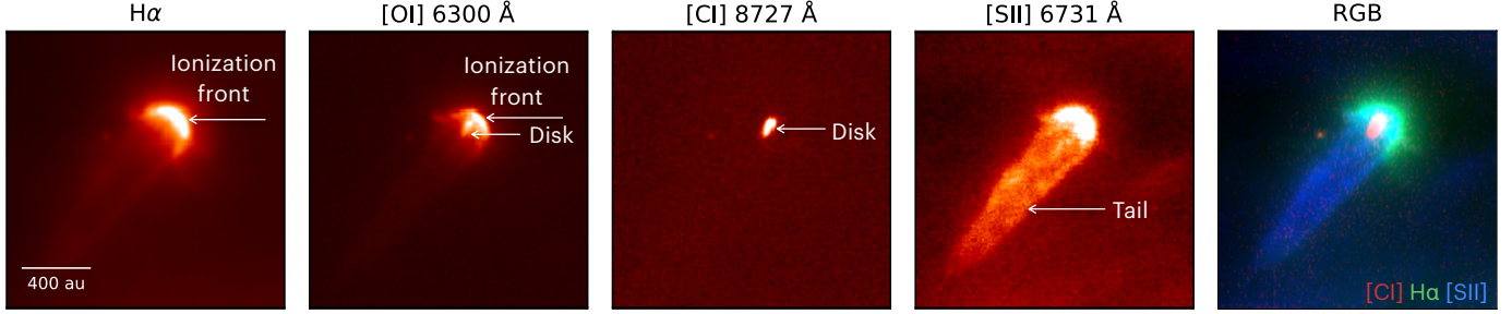
Fig. 5. Continuum-subtracted, single-line integrated flux images and an RGB image of proplyd 177–341W. The panels show which parts of the system are visible in given emission lines.
