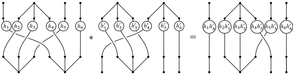
Figure 6. Multiplication of spraiges.
