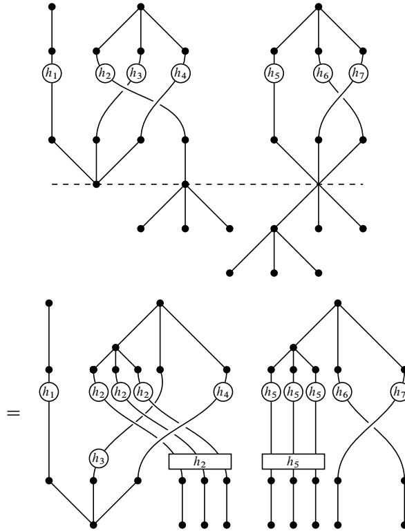
Figure 8. A splitting of a spraige.
