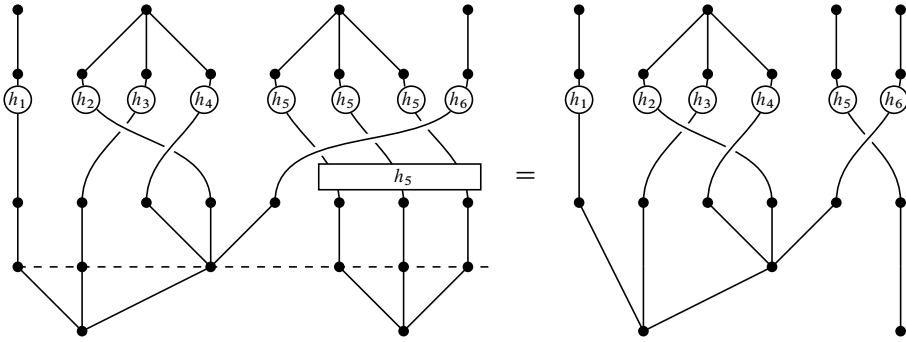
Figure 9. An elementary merging of a sprai.
