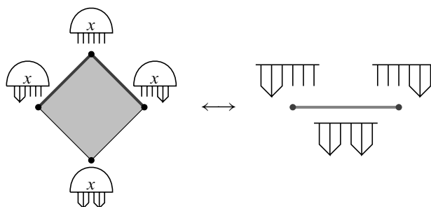
Figure 11. The correspondence between \text{Lk}\downarrow(x) and \mathcal{E}\mathcal{B}_d^m .
