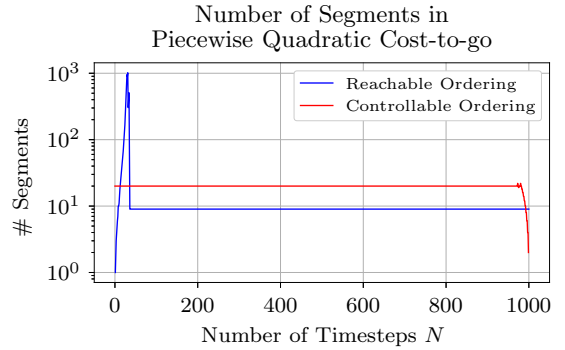
Fig. 9. The number of segments in the piecewise quadratic cost-to-go functions for each time step remains mostly constant throughout the optimization. The rapid growth followed by decay for the reachable ordering explains the apparent non-zero y-intercept in Fig. 8.
