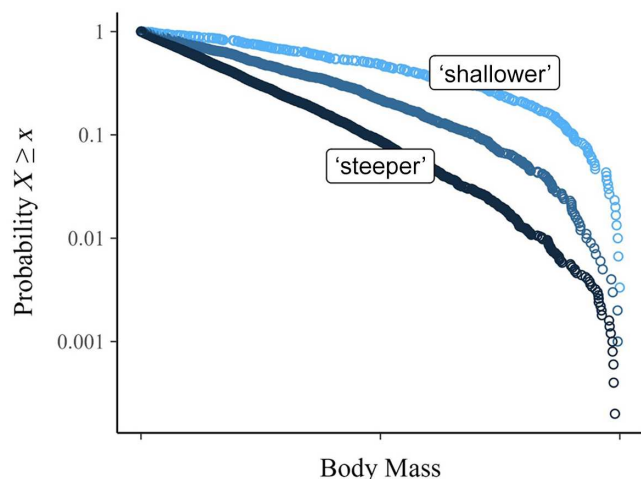
FIGURE 2 Community size spectra showing hypothetical change from the normal state (middle) to a “shallower” slope or “steeper” of the slope. Overfishing results in a steepening of the community size spectra (CSS) (Kolding et al., 2016; Sweeting et al., 2009; Wilson et al., 2010), while dominance of large-bodied, low trophic position fish will tend to flatten the line (Broadway et al., 2015; Murry et al., 2024). The data points are individual body sizes of fish with truncation at the smallest and largest fish. The y-axis is the probability of a body size being greater than or equal to a given body size. The shape of these curves is governed by the parameter \lambda in individual size distributions (ISD; see CSS methodology section below for details).
