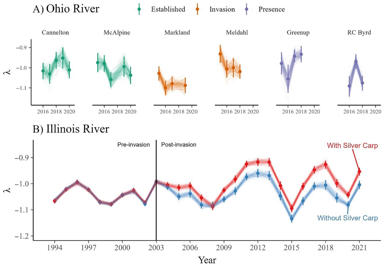
FIGURE 4 Time series of \lambda in (A) six pools of the Ohio River and (B) the Illinois River. Data points show the median and 95% CrI based on varying intercepts from the generalized linear mixed model. An exception are the data points and lines in (B) “Without Silver Carp.” These come from a separate model with year as a fixed effect and Silver Carp excluded from the body size data. Lines connecting the data points show 100 draws from the posterior distribution to aid in visual interpretation.
