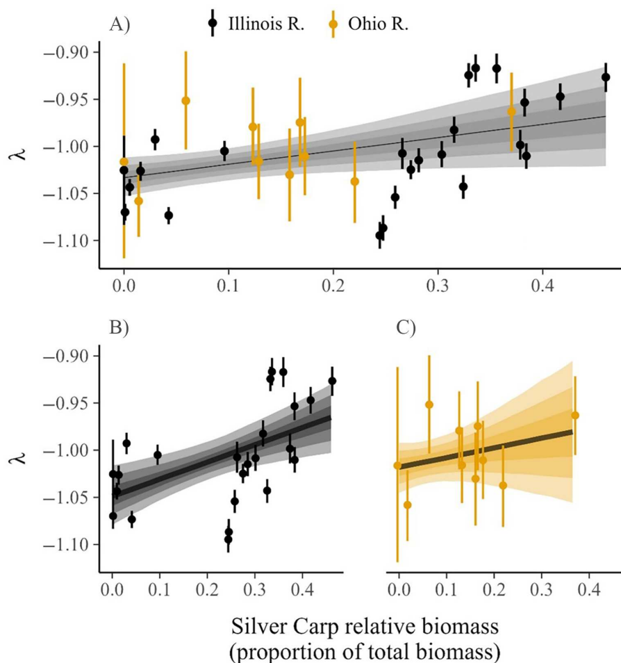
FIGURE 3 Relationship between community size spectra ( \lambda ) and Silver Carp invasion. (A) The model outcome averaged over both rivers; (B, C) the conditional model outcomes for each river separately. Regression lines show the median (black) regression. Shading shows the 50%, 80%, and 95% credible intervals (CrIs). Data points are the varying intercept estimates for each sample ( \pm 95\% CrI).
