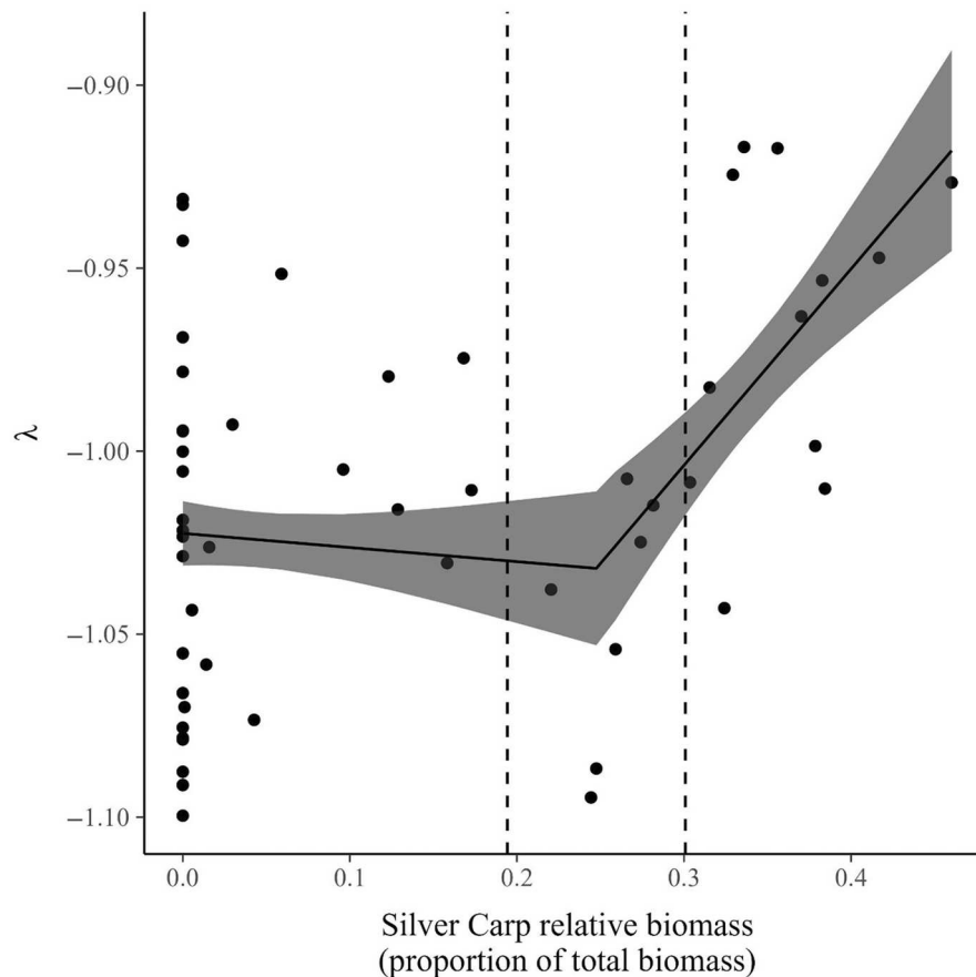
FIGURE 5 Results of a segmented regression between lambda and silver carp relative biomass. The data points are the posterior mean lambdas, obtained from the varying intercepts of the full truncated Pareto model. The regression line and shaded area show the fitted relationship between lambda and silver carp relative biomass below and above the threshold. The dashed lines indicate one SD below and above the mean threshold estimate of 0.24.
