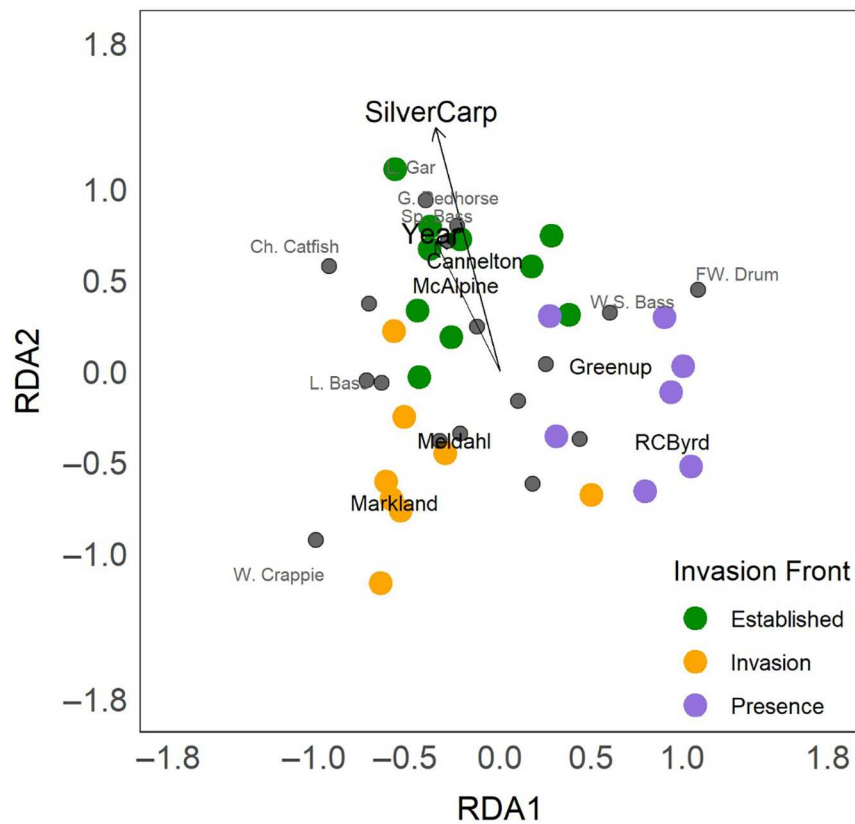
FIGURE 7 Redundancy analysis (RDA) results for the Ohio River. Silver Carp catch per unit effort (CPUE), Pool (from downstream to upstream: Cannelton, McAlpine, Markland, Meldahl, Greenup, RC Byrd), and Year were the main effects. Silver Carp CPUE and Year were not significant, but differences in fish assemblage were related to pool. The gray circles depict individual species.
