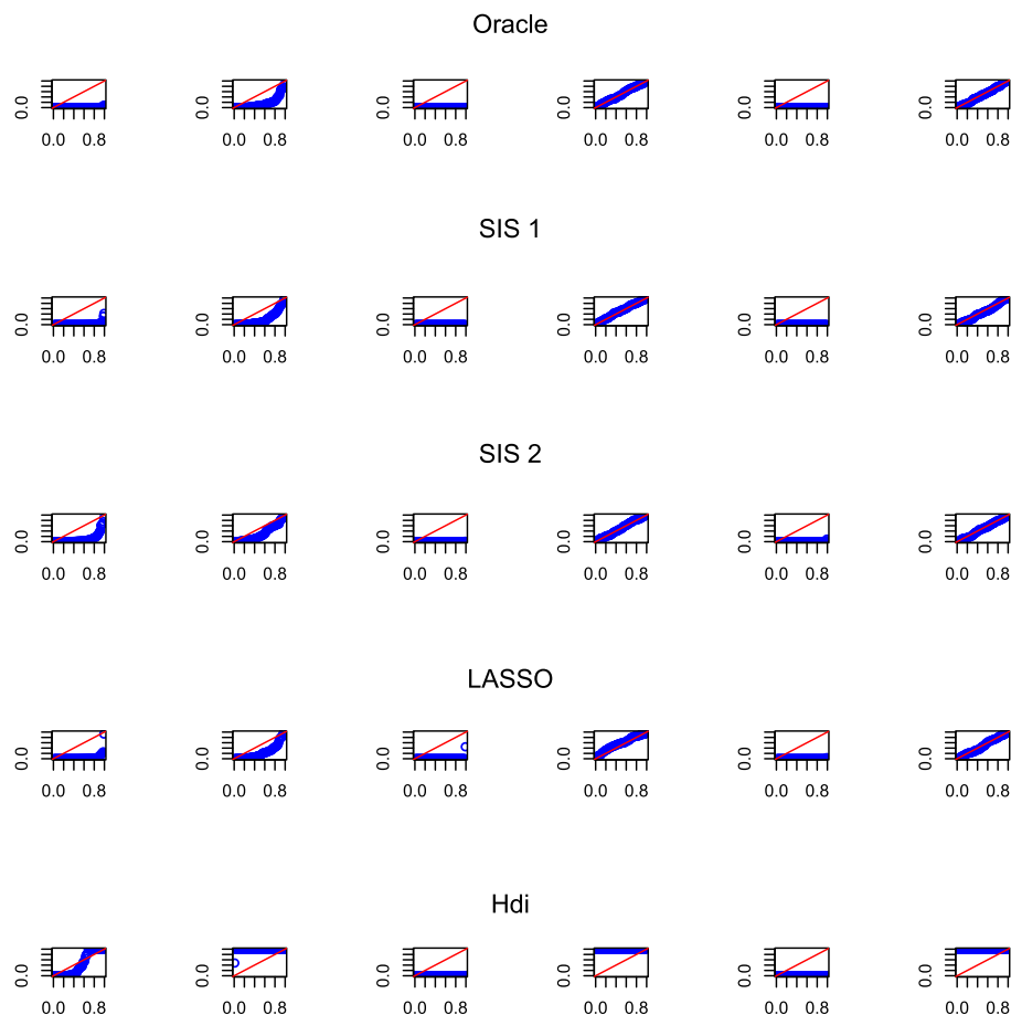
FIG 3. The Q-Q plots of P-values estimated in Example 3 by various procedures: the proposed oracle P-values, SIS-1, SIS-2, LASSO, and hdi. In each row, each column (from left to right) corresponds to the Q-Q plot for one variable in \{X_1, \dots, X_6\} , respectively. Recall that X_1, X_2, X_3, X_5 are important variables, and X_4 and X_6 are noise variables. In each plot, the x-axis represents the theoretical quantiles of Unif(0, 1) , and the y-axis represents the observed quantiles for the calculated P-values.
