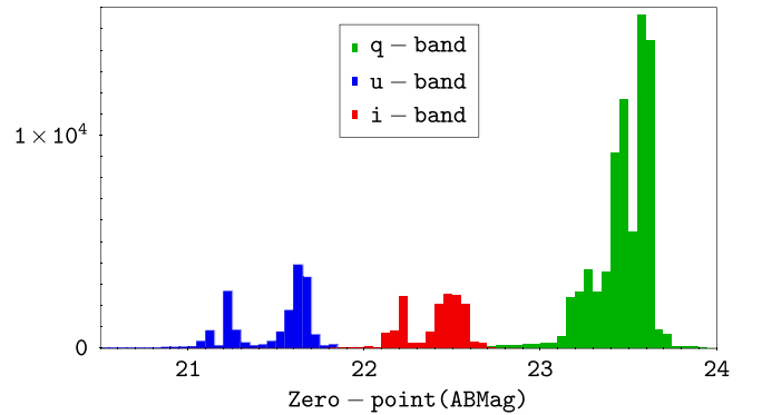
Figure 14. Distribution of measured zero-points in the u (blue), q (green) and i -bands (red) on BG4 over the period 2023 April 1 to 2024 October 20.
