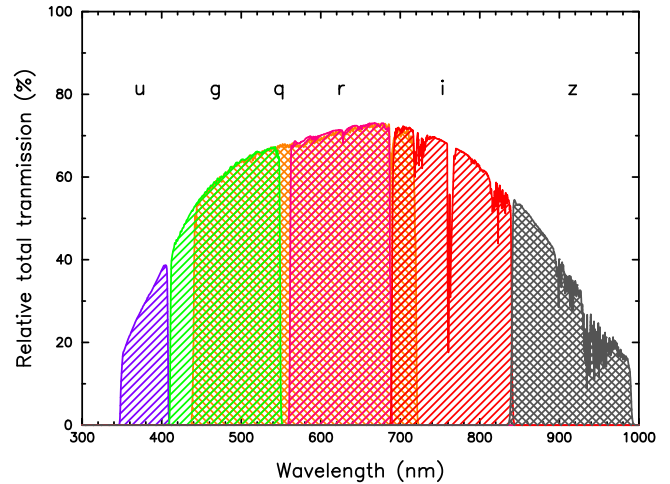
Figure 6. Overall relative transmission of the BlackGEM telescope system, from the top of the atmosphere to the detector, as a function of wavelength. Color coding as in Figure 2.
