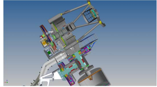
Figure 10. Cut-open view of the BlackGEM telescope on the Fornax 200 mount, also showing the drum-shaped counter-weight and the fly-over cable wrap.
