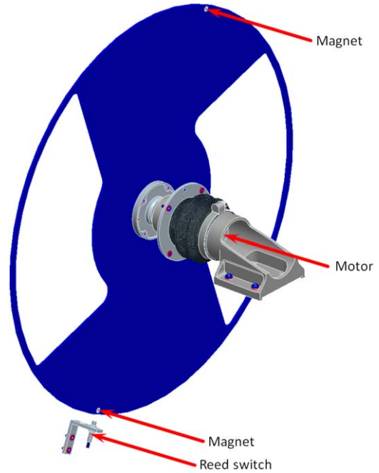
Figure 9. Butterfly design of the BlackGEM shutter, showing the curved sides that ensure equal illumination per pixel during opening and closing of the shutter.
