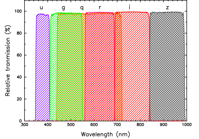
Figure 2. Transmission curves of the BlackGEM filters. Purple is the u -band, green the g -band, orange the q -band, red the r -band, light-red the i -band and in gray the z -band.
