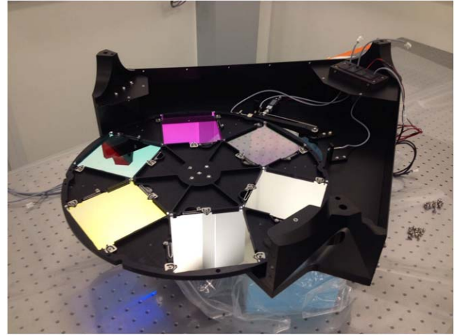
Figure 3. Photo of the opened filter wheel during assembly.
