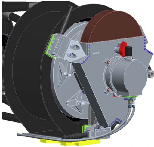
Figure 8. Backside view of the mechanical design of the BlackGEM telescope. At the far left, the carbon-fiber mirror cell (black) can be seen with the main mirror (gray) supported on an 18-point, 6-pad, 3-arm whiffle tree. The shutter/filterwheel housing and the cryostat (brown/gray) are attached to the carbon fiber mirror cell on three spring-blade clamping points (green). The attachment to the mount is via an interface plate, which is part of the carbon-fiber mirror cell (yellow).
