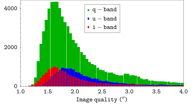
Figure 13. Distribution of measured image quality in the u (blue), q (green) and i -bands (red) on BG4 over the period 2023 April 1 to 2024 October 20.
