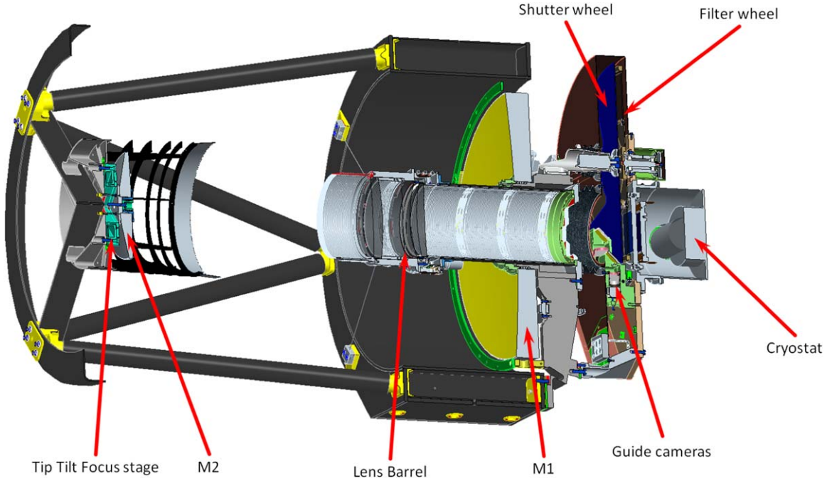
Figure 7. Annotated design drawing of the BlackGEM telescopes.
