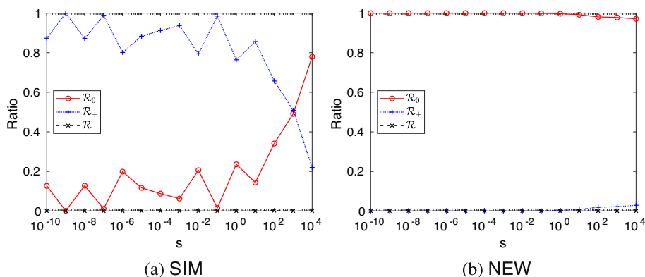
Fig. 2 Example 1. Ratios \mathcal{R}_0 , \mathcal{R}_+ , and \mathcal{R}_- for correct, over, and under detections, respectively, among 1000 randomly selected intervals of size s
