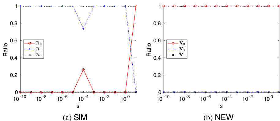
Fig. 5 Example 2. Ratios \mathcal{R}_0 , \mathcal{R}_+ , and \mathcal{R}_- for correct, over, and under detections, respectively, among 1000 runs each with a different random vector z
