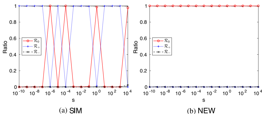
Fig. 3 Example 1. Ratios \mathcal{R}_0 , \mathcal{R}_+ , and \mathcal{R}_- for correct, over, and under detections, respectively, among 1000 runs each with a different random vector z
