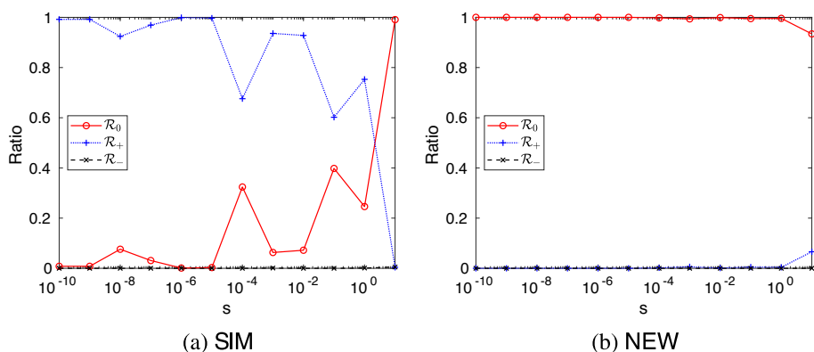
Fig. 4 Example 2. Ratios \mathcal{R}_0 , \mathcal{R}_+ , and \mathcal{R}_- for correct, over, and under detections, respectively, among 1000 randomly selected intervals of size s
