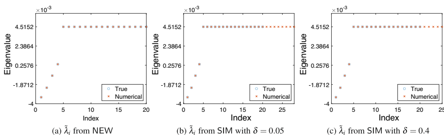
Fig. 6 Example 2. Numerical eigenvalues (x) \tilde{\lambda}_i within (-0.004, 0.00451518) from NEW and SIM
